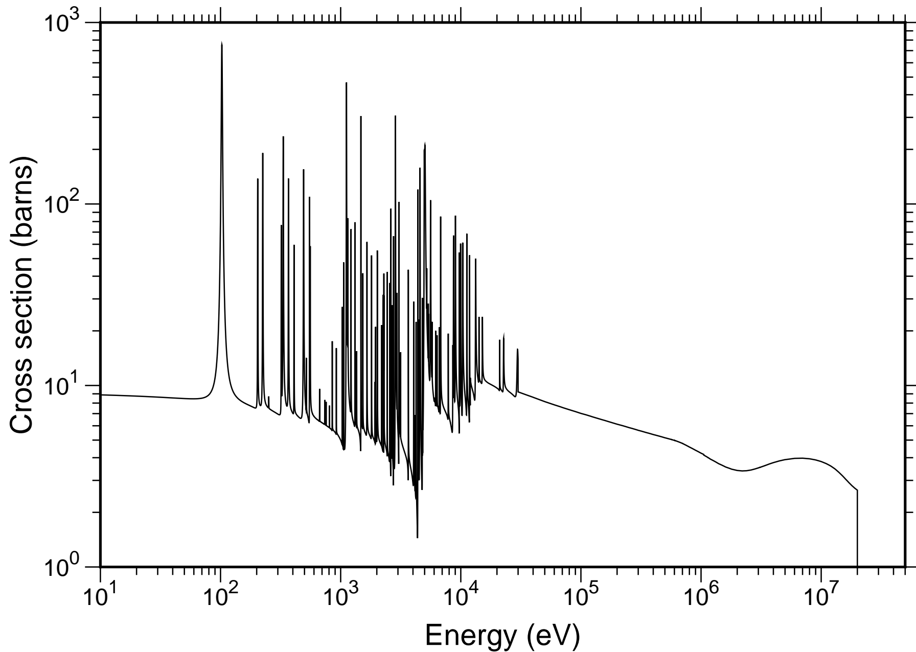
Natural Ge Total Cross-section - JENDL-4.0
