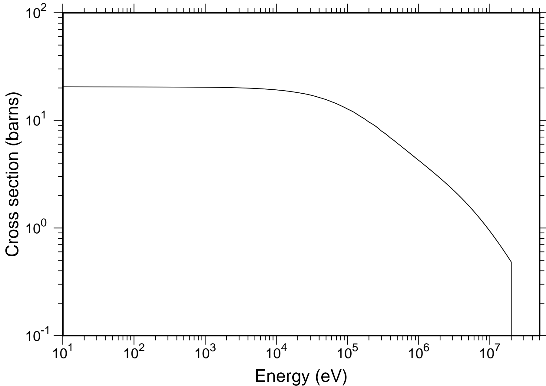
Natural H Total Cross-section - JENDL-4.0
