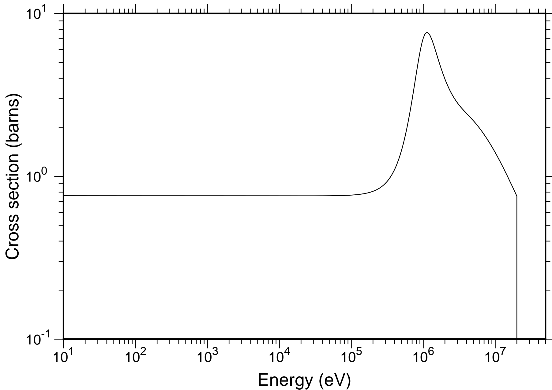
Natural He Total Cross-section - JENDL-4.0
