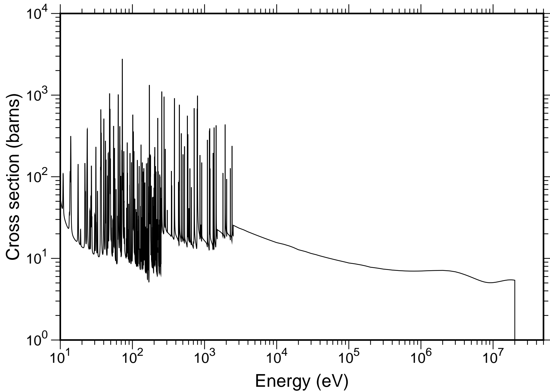
Natural Hf Total Cross-section - JENDL-4.0
