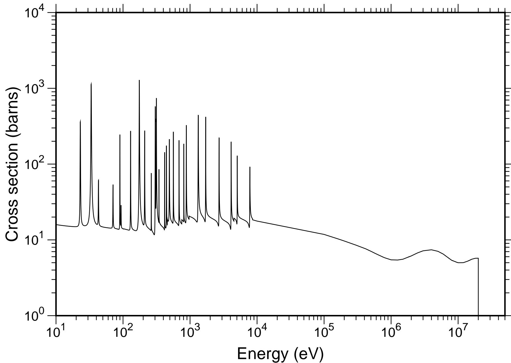
Natural Hg Total Cross-section - JENDL-4.0
