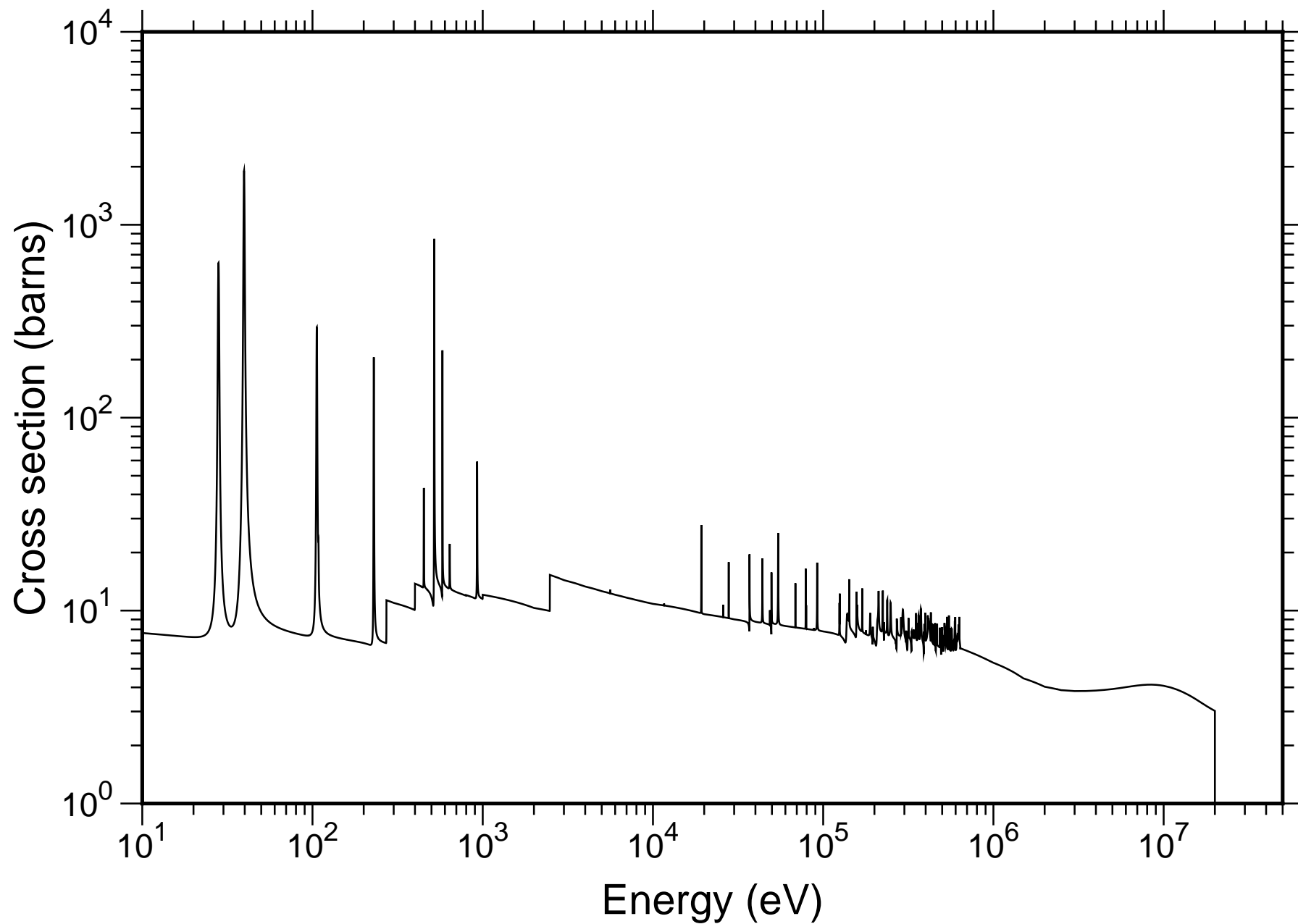
Natural Kr Total Cross-section - JENDL-4.0
