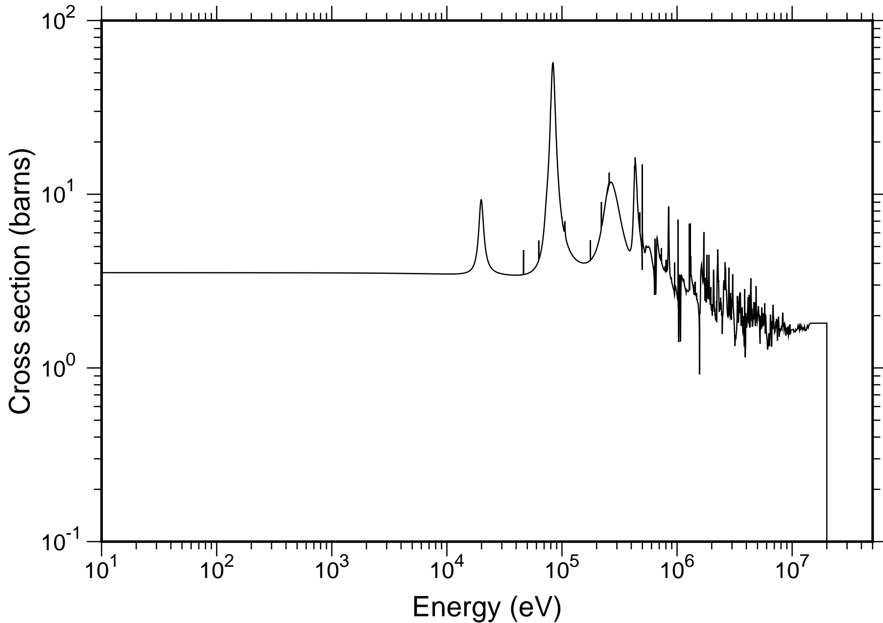
Natural Mg Total Cross-section - JENDL-4.0
