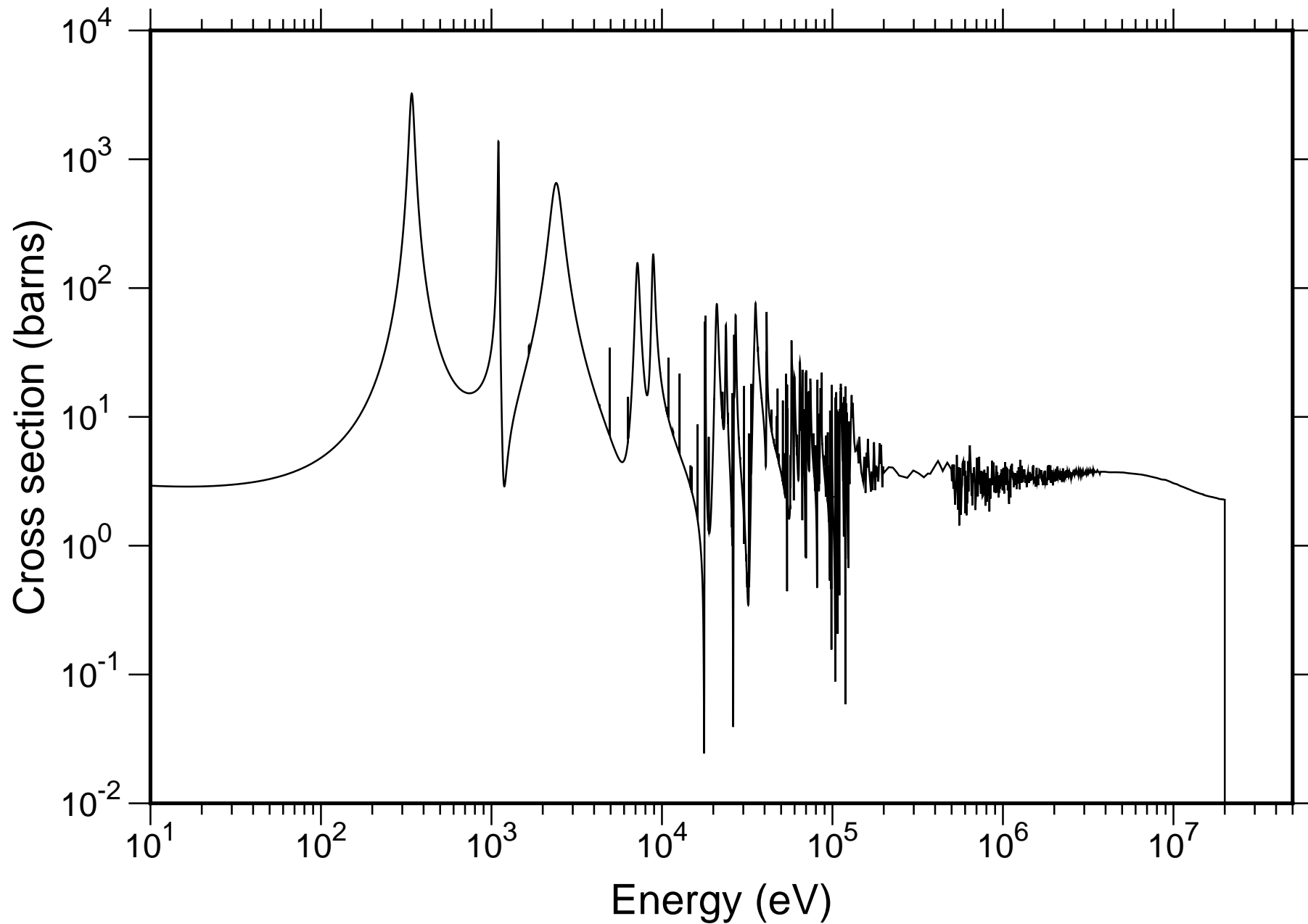
Natural Mn Total Cross-section - JENDL-4.0
