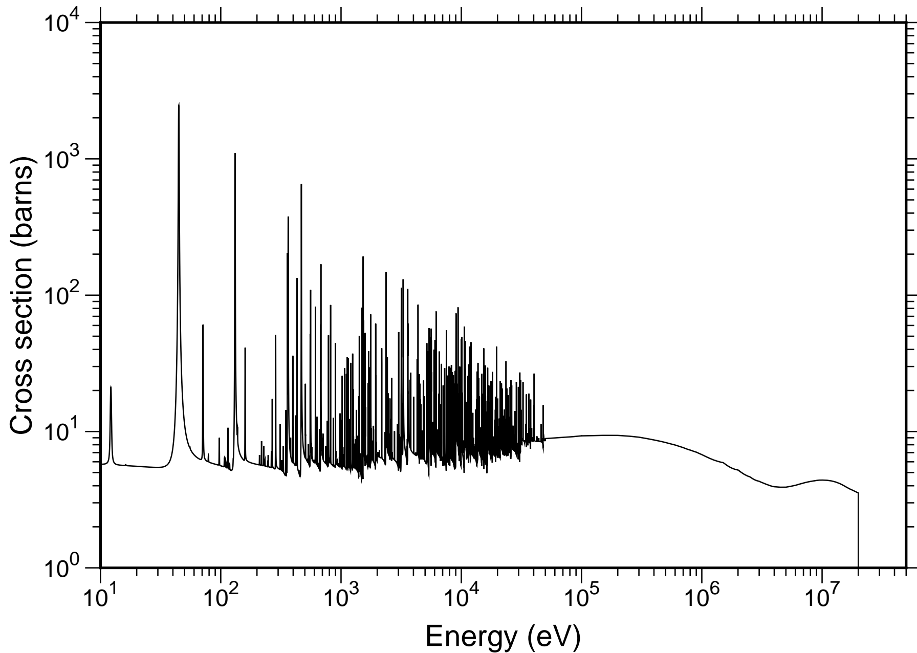
Natural Mo Total Cross-section - JENDL-4.0
