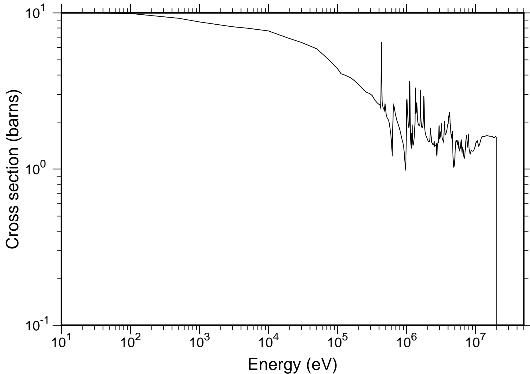
Natural N Total Cross-section - JENDL-4.0
