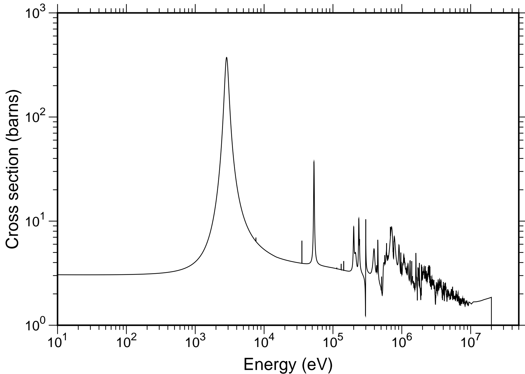
Natural Na Total Cross-section - JENDL-4.0
