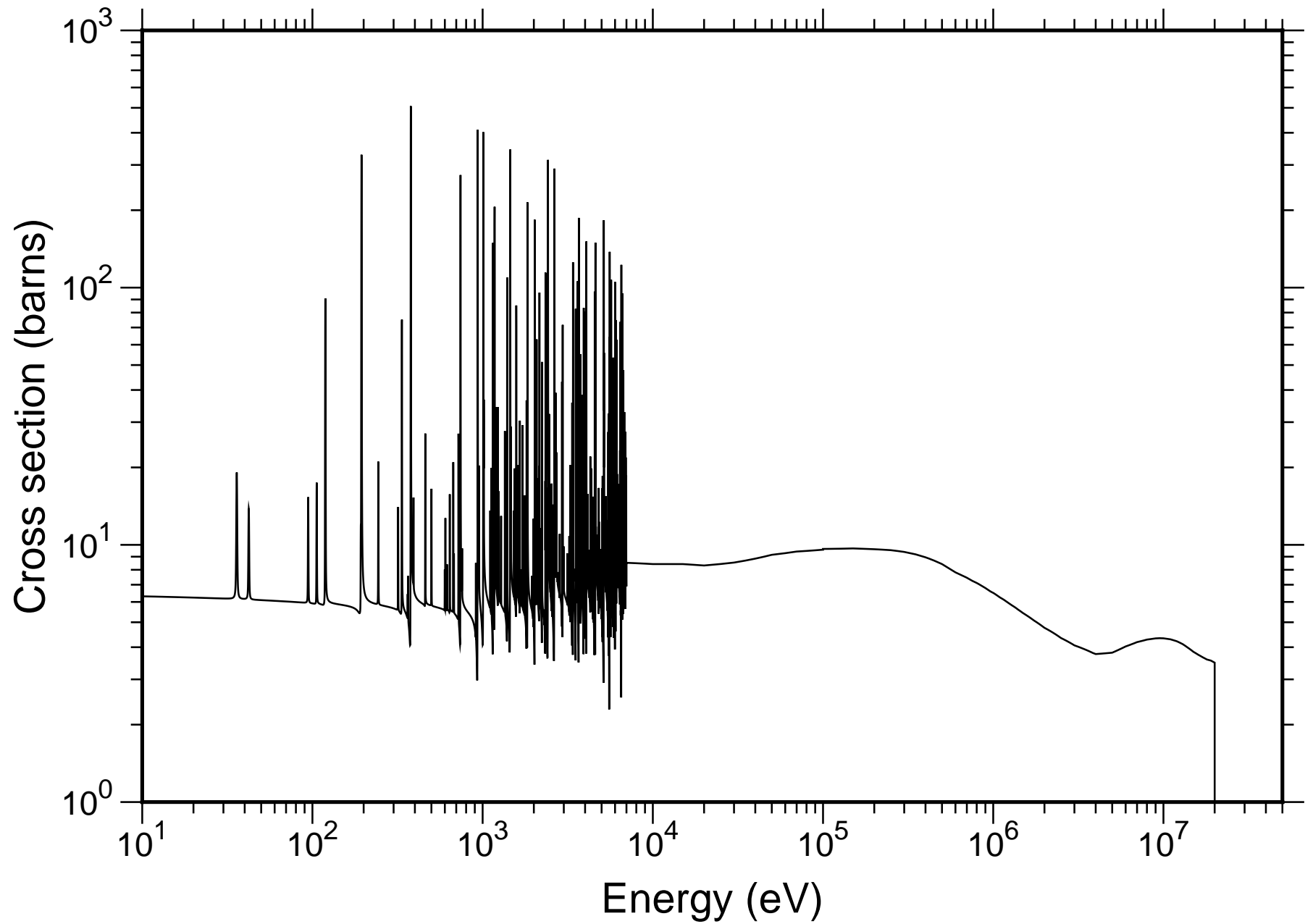
Natural Nb Total Cross-section - JENDL-4.0
