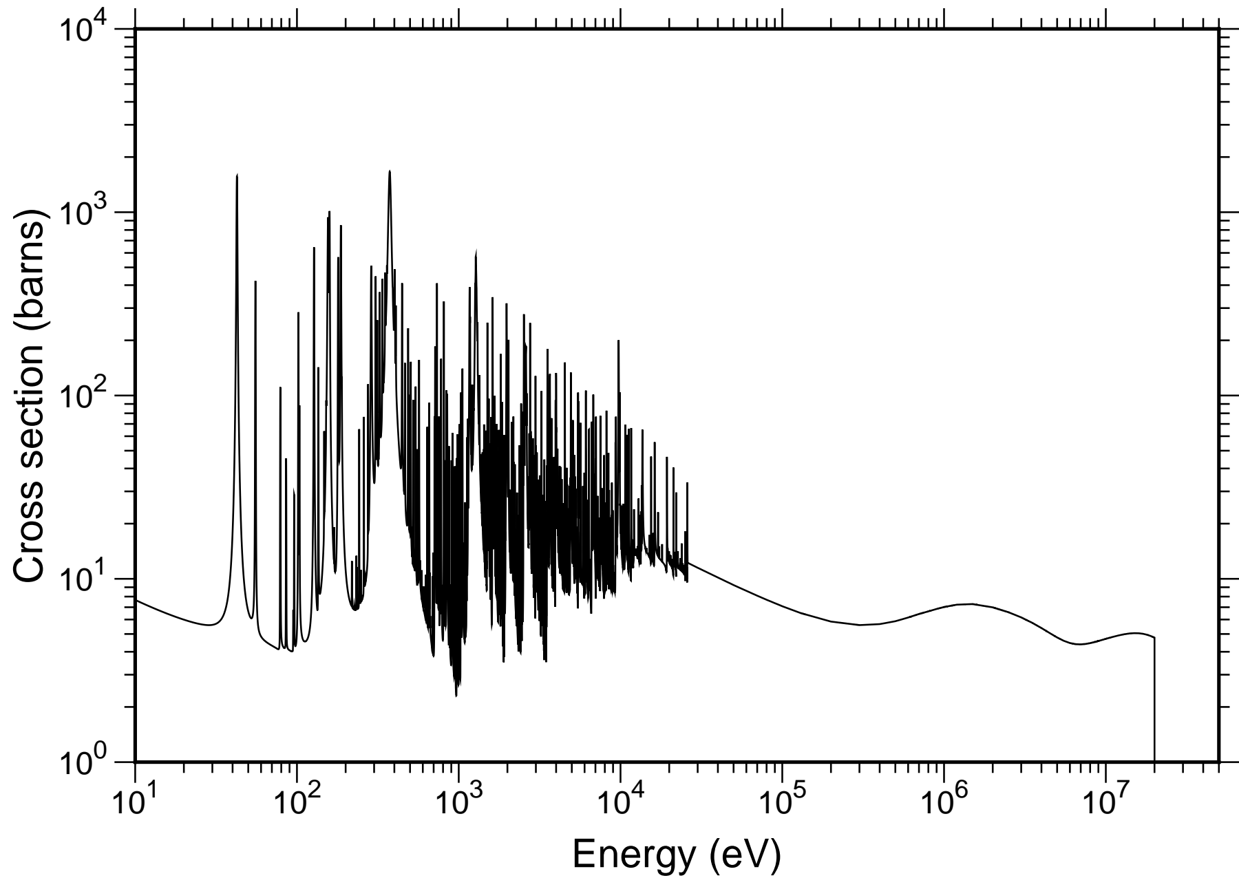
Natural Nd Total Cross-section - JENDL-4.0
