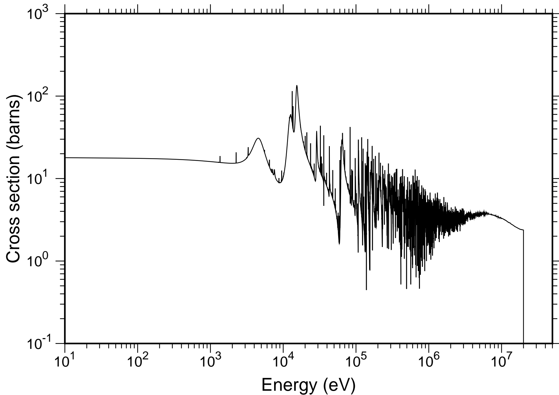
Natural Ni Total Cross-section - JENDL-4.0
