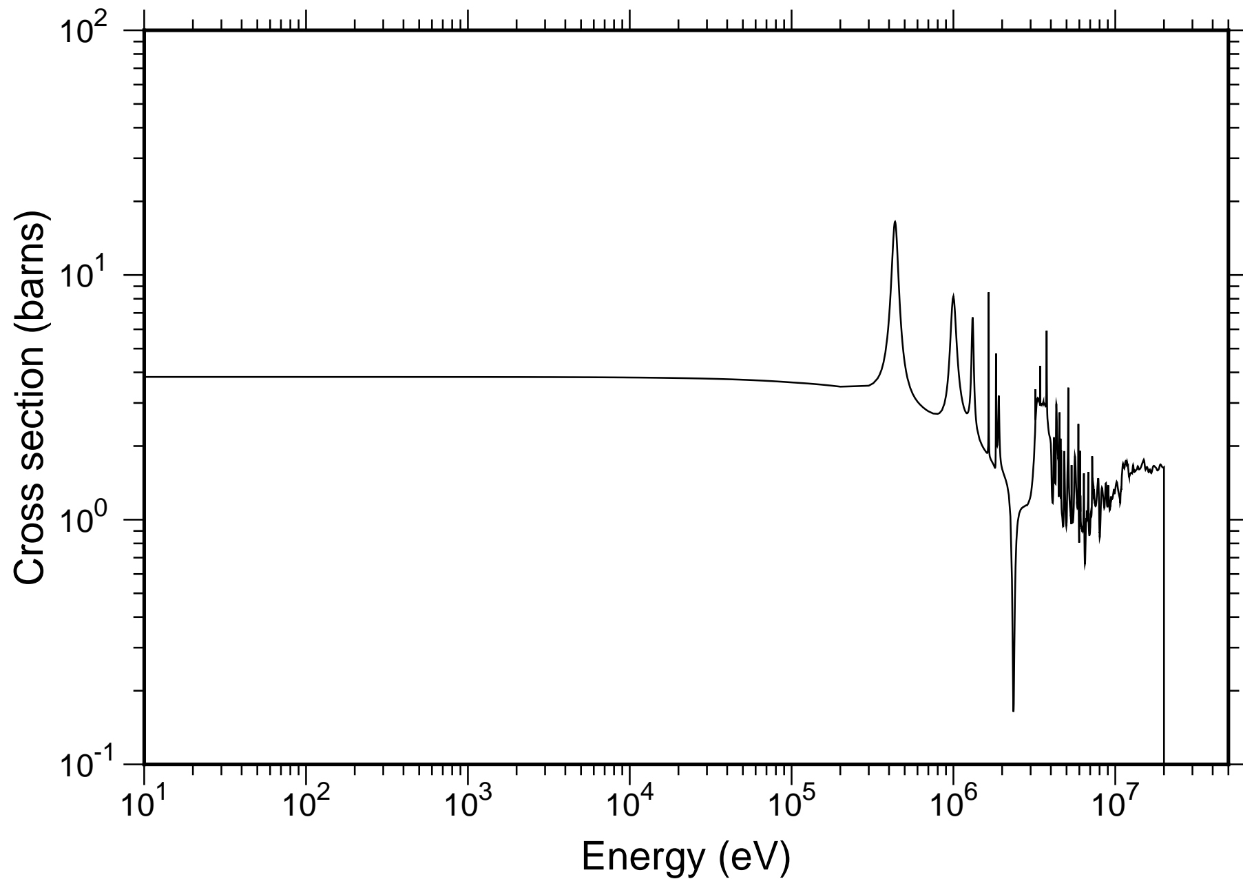
Natural O Total Cross-section - JENDL-4.0
