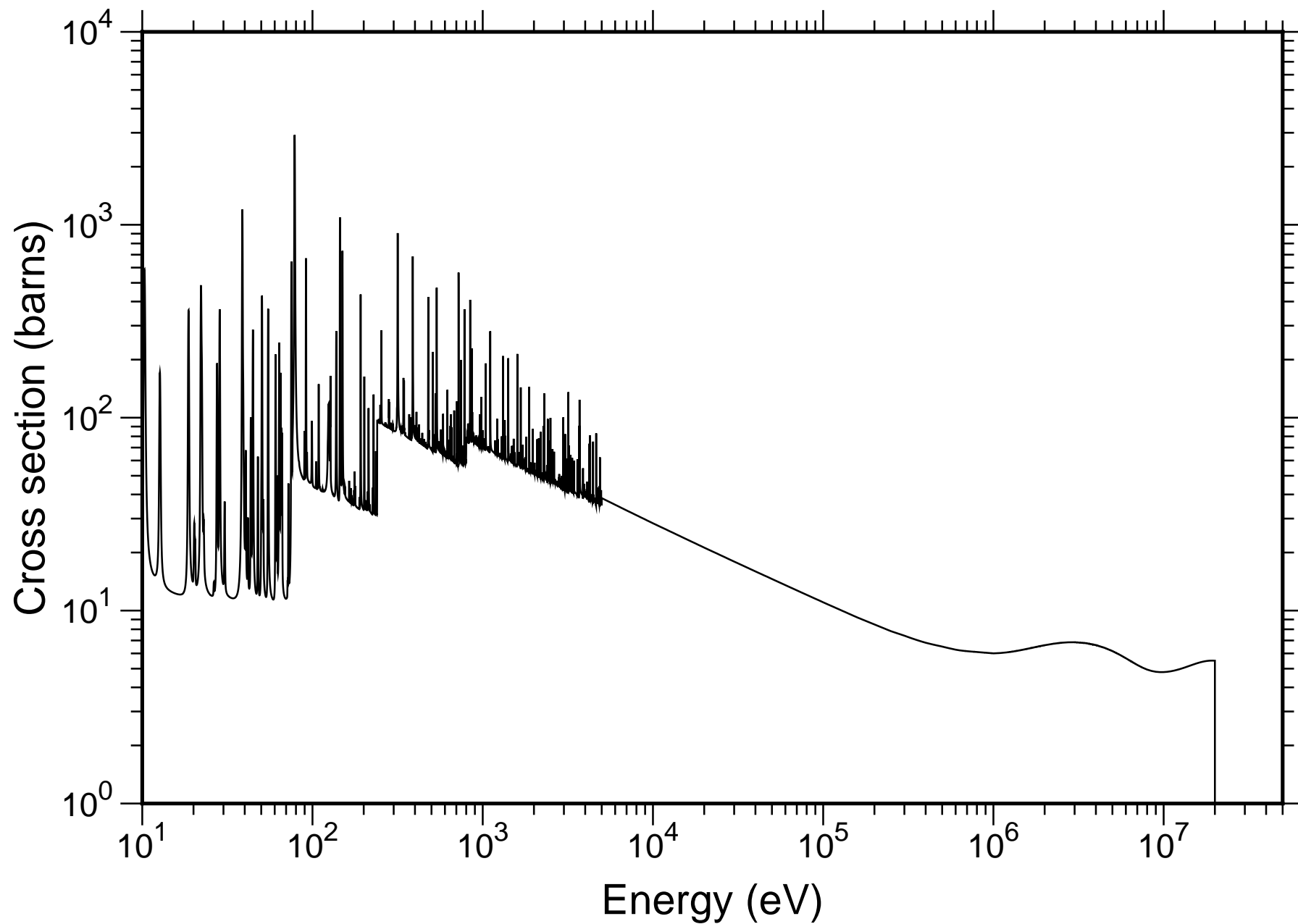
Natural Os Total Cross-section - JENDL-4.0
