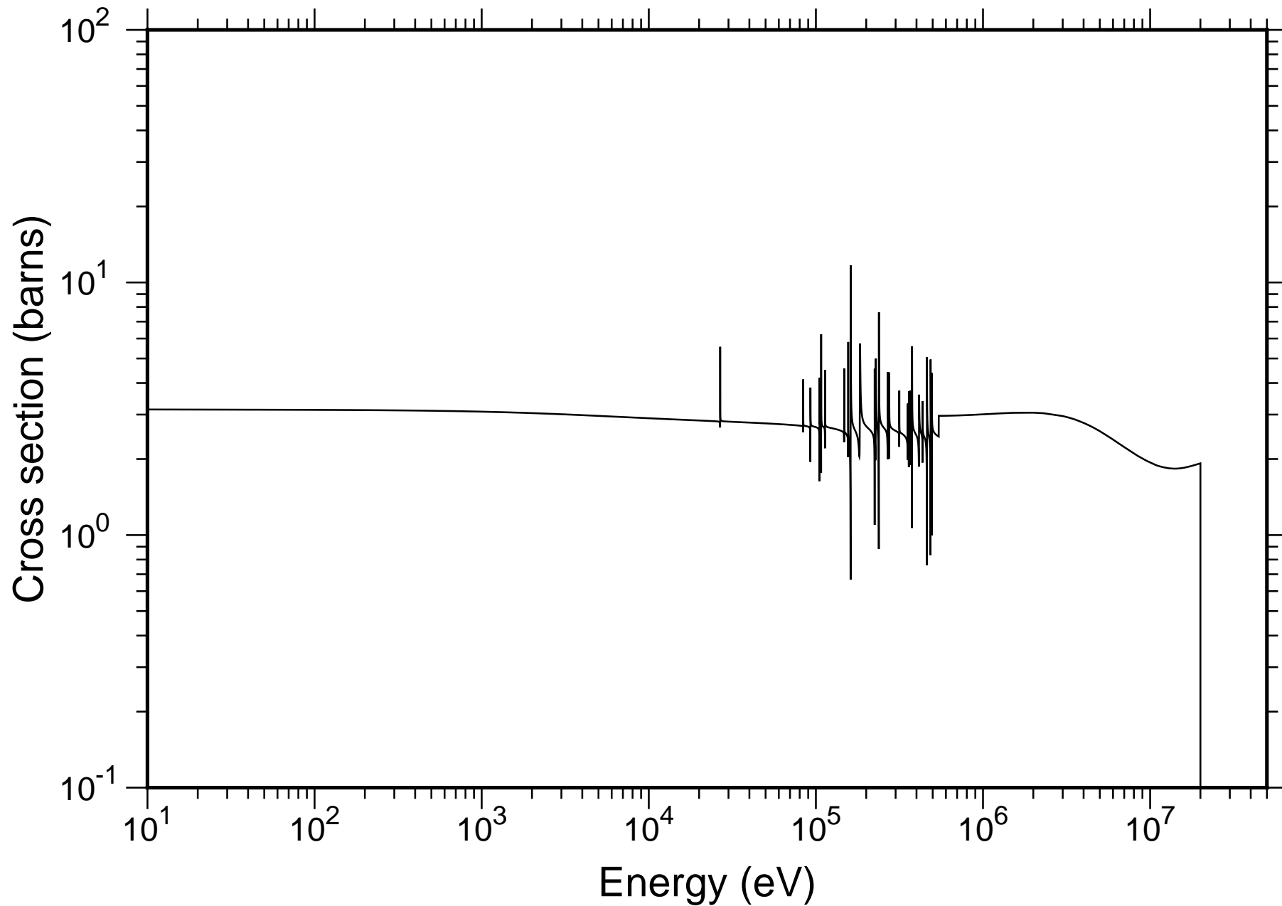
Natural P Total Cross-section - JENDL-4.0
