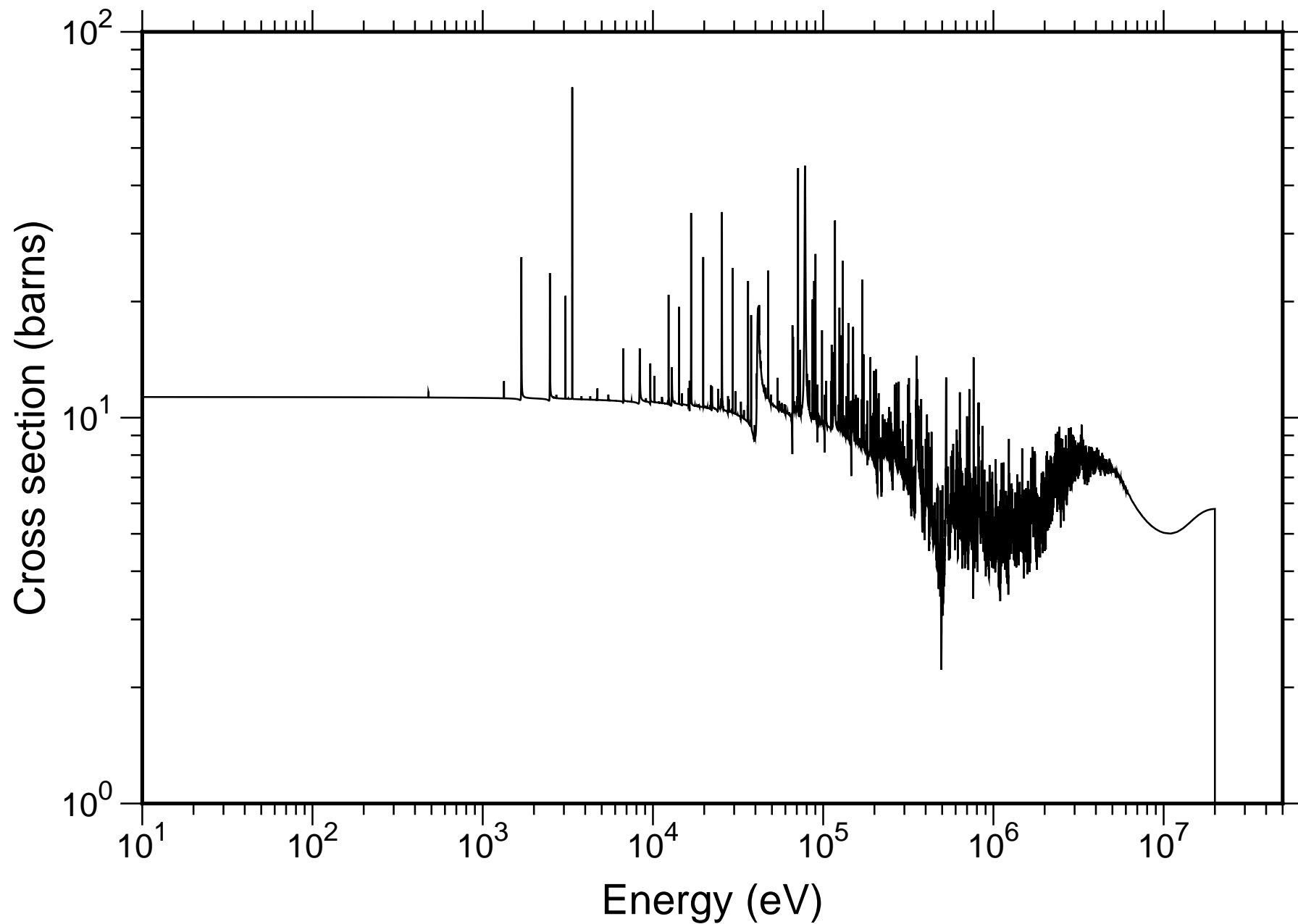
Natural Pb Total Cross-section - JENDL-4.0
