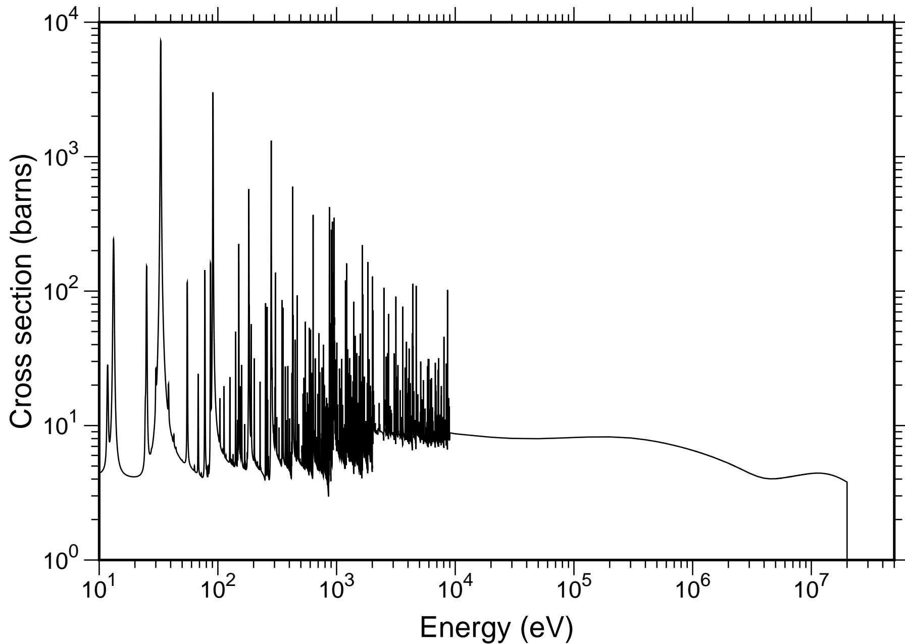
Natural Pd Total Cross-section - JENDL-4.0
