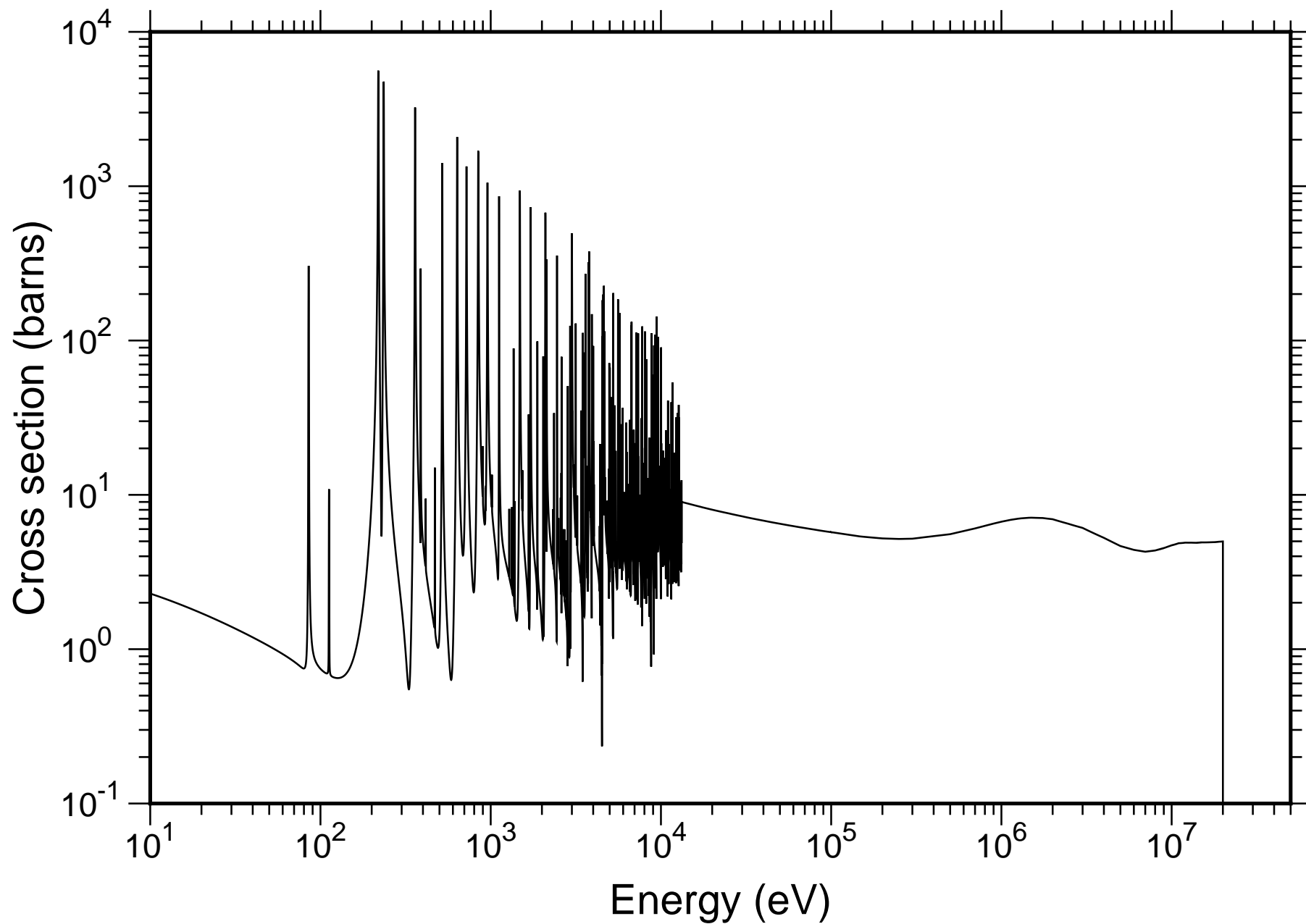
Natural Pr Total Cross-section - JENDL-4.0
