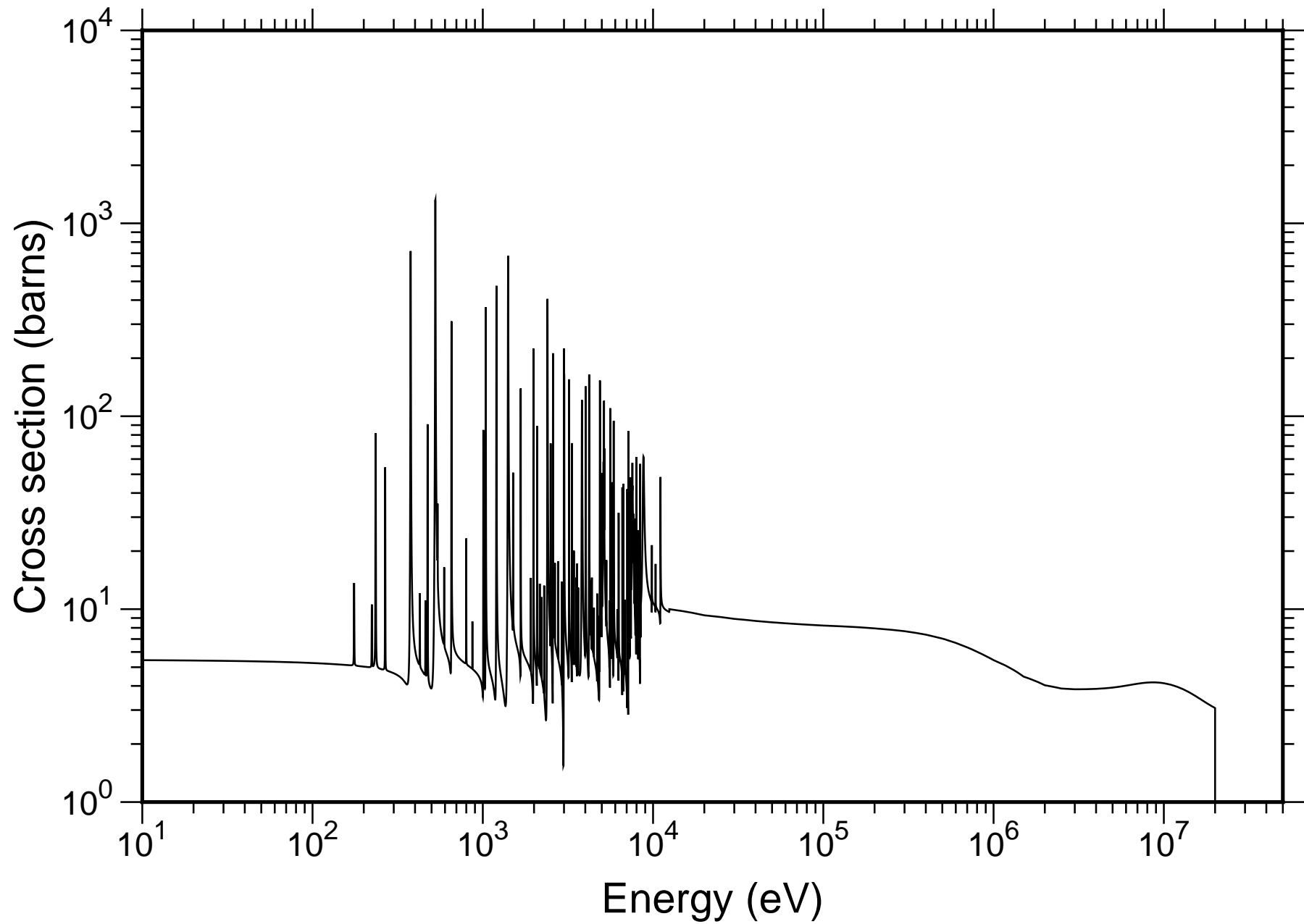
Natural Rb Total Cross-section - JENDL-4.0
