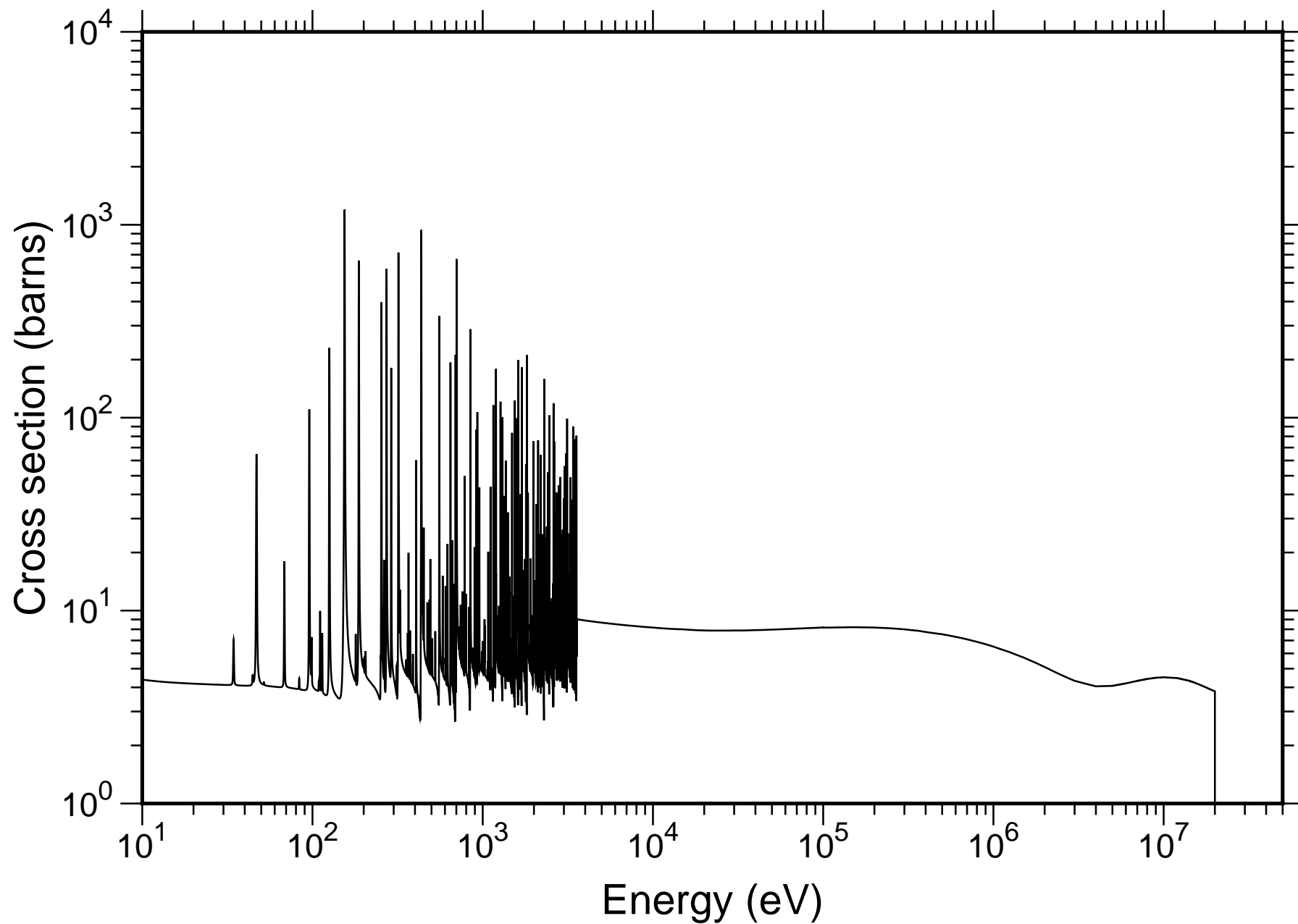
Natural Rh Total Cross-section - JENDL-4.0
