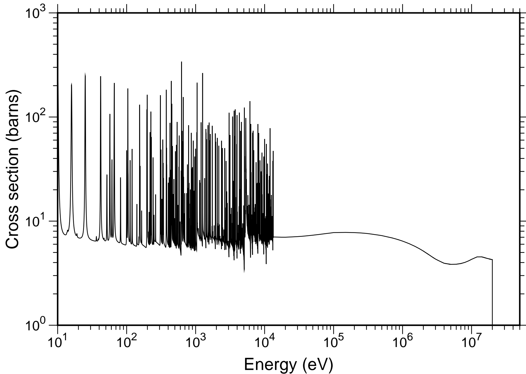
Natural Ru Total Cross-section - JENDL-4.0
