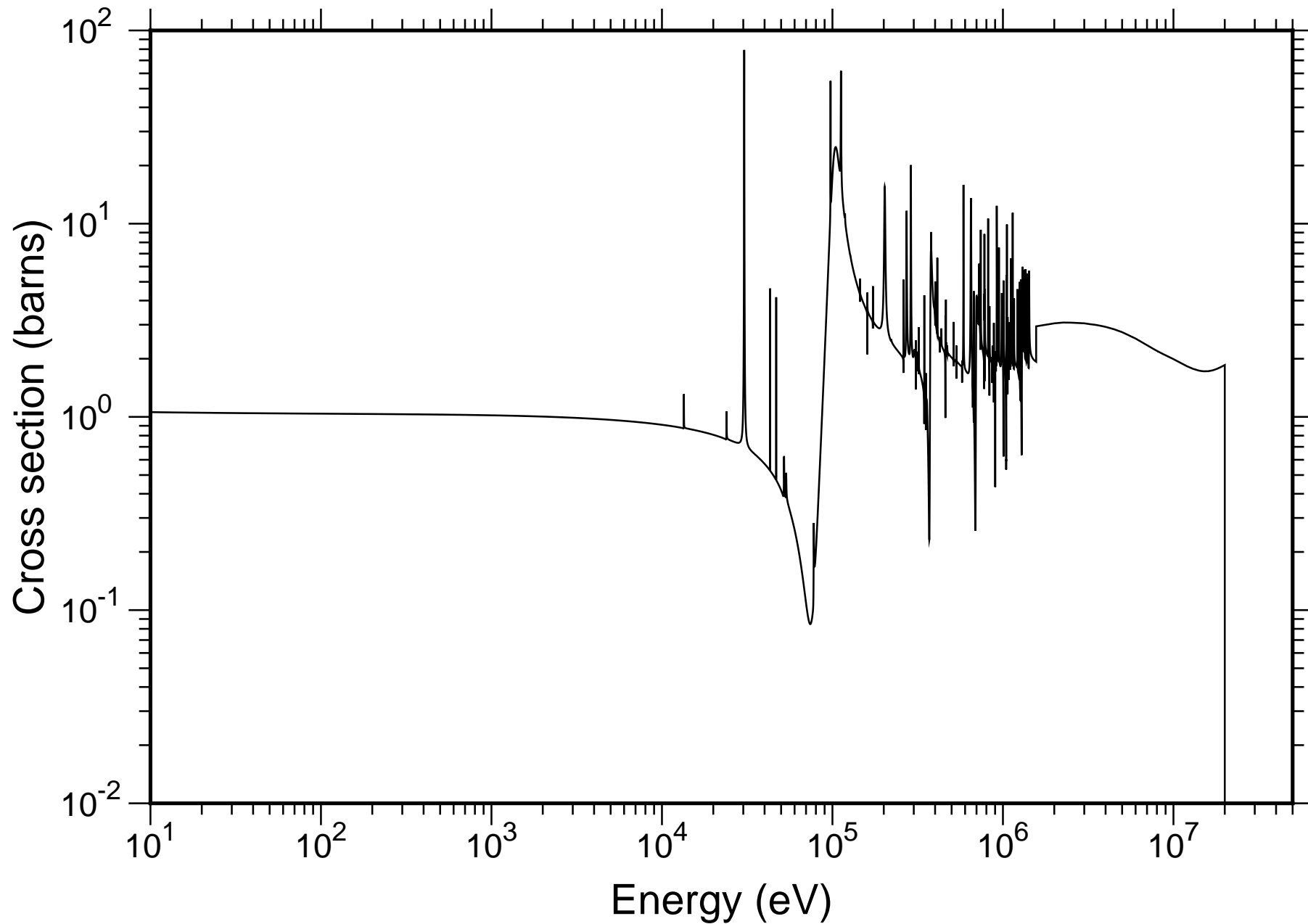
Natural S Total Cross-section - JENDL-4.0
