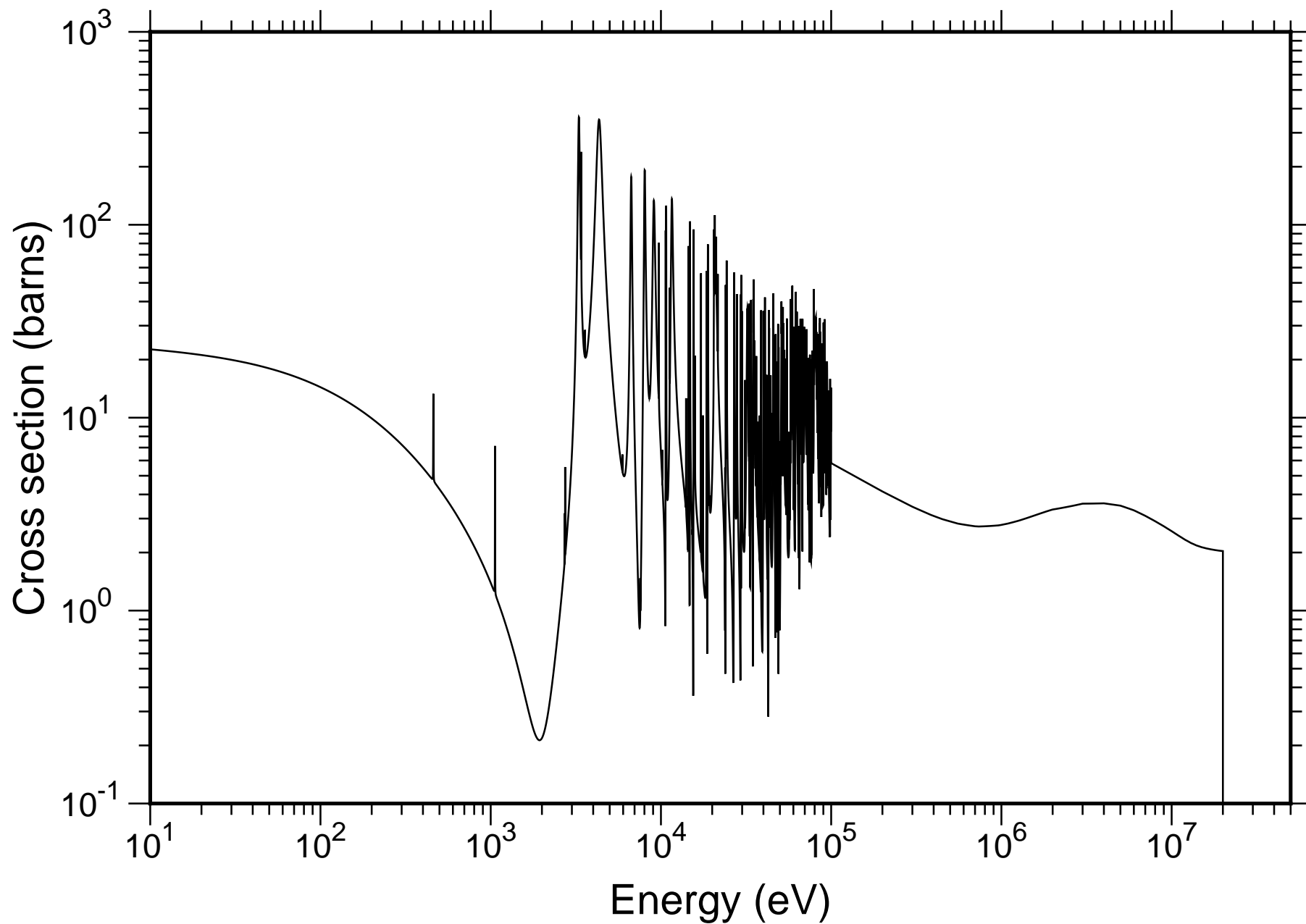
Natural Sc Total Cross-section - JENDL-4.0
