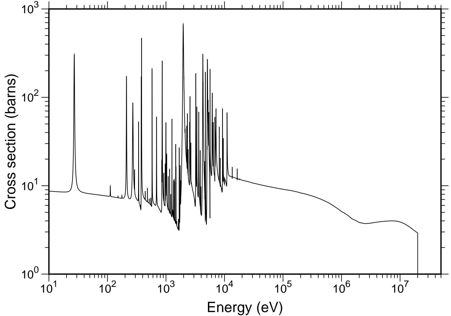
Natural Se Total Cross-section - JENDL-4.0
