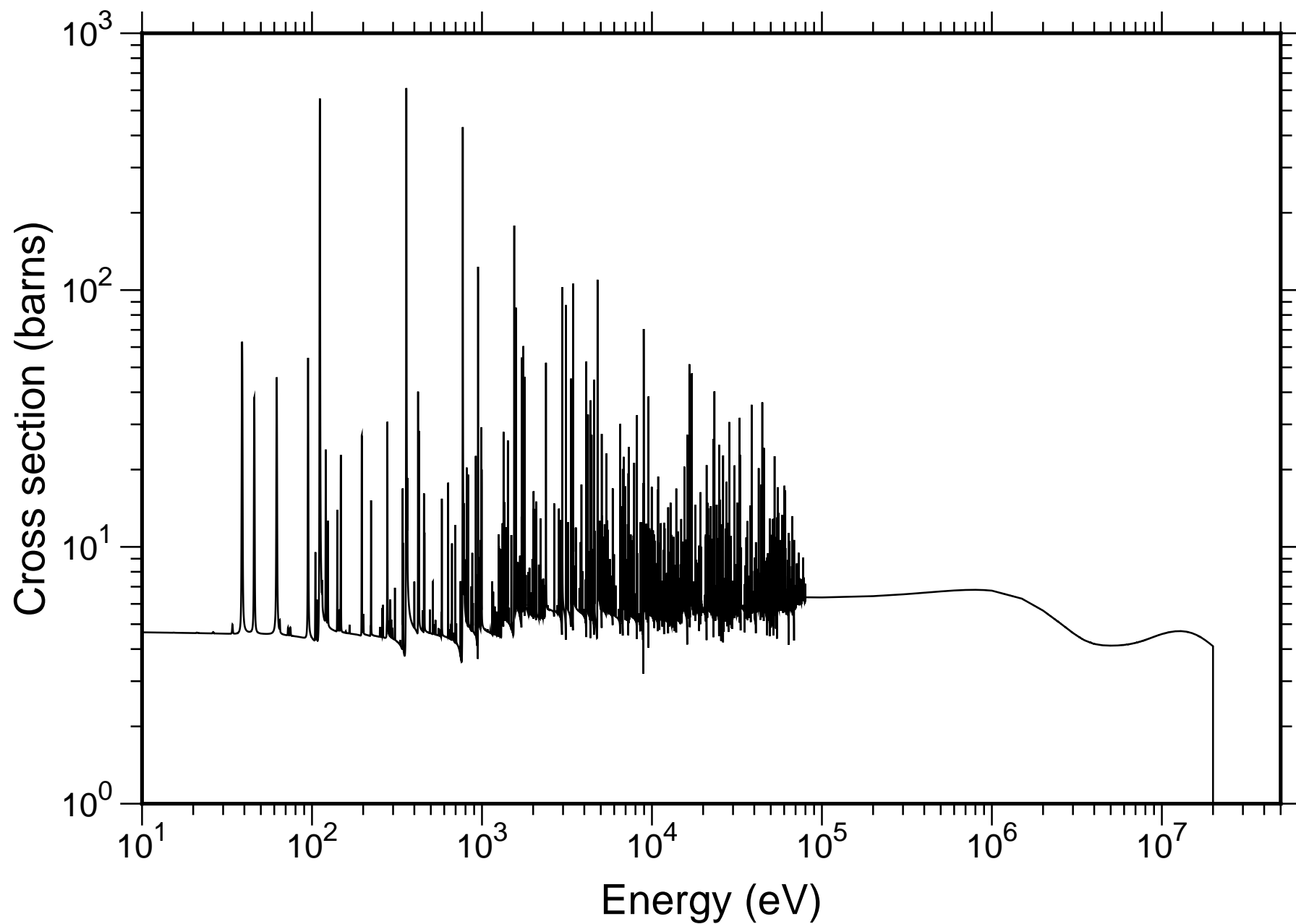
Natural Sn Total Cross-section - JENDL-4.0
