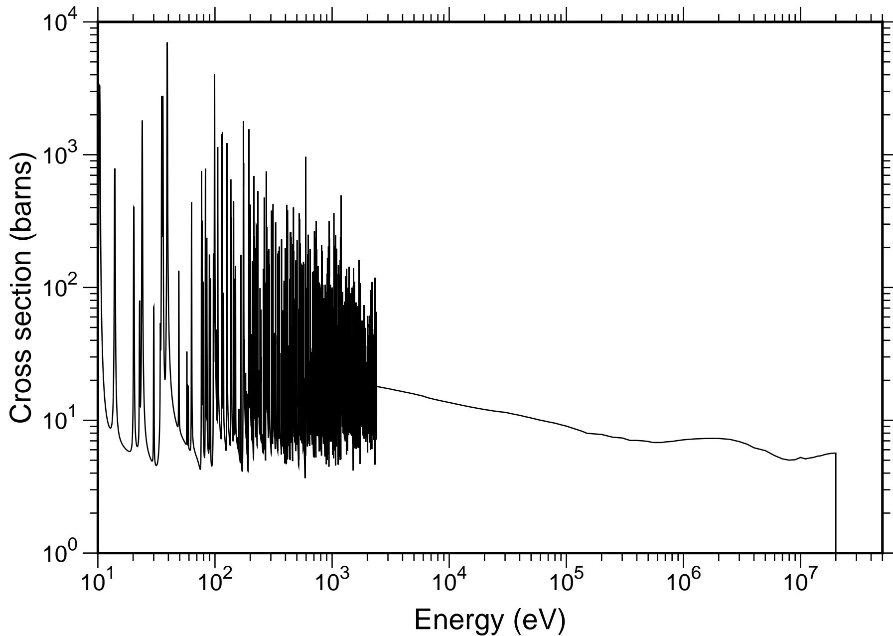
Natural Ta Total Cross-section - JENDL-4.0
