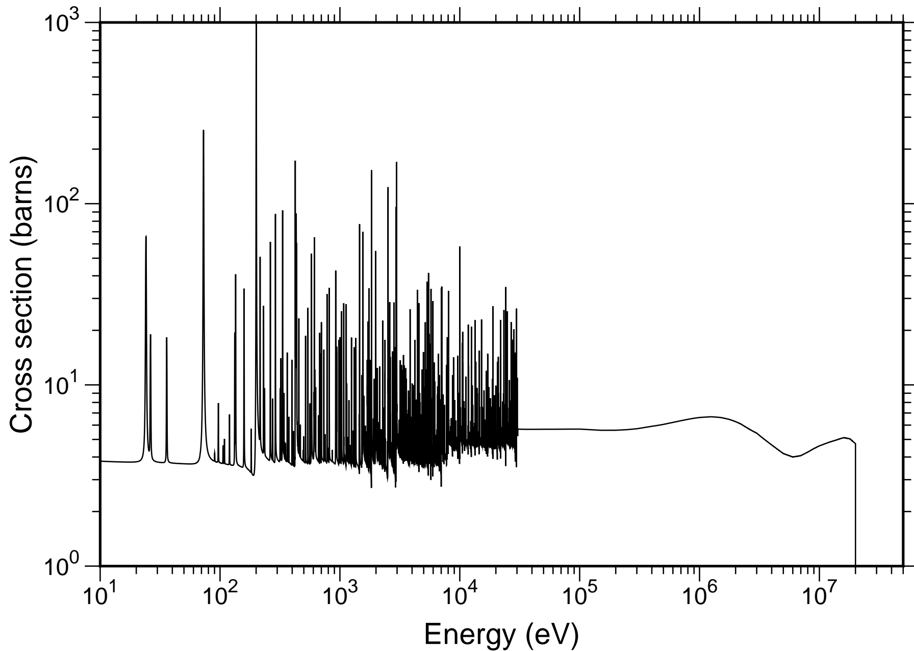
Natural Te Total Cross-section - JENDL-4.0
