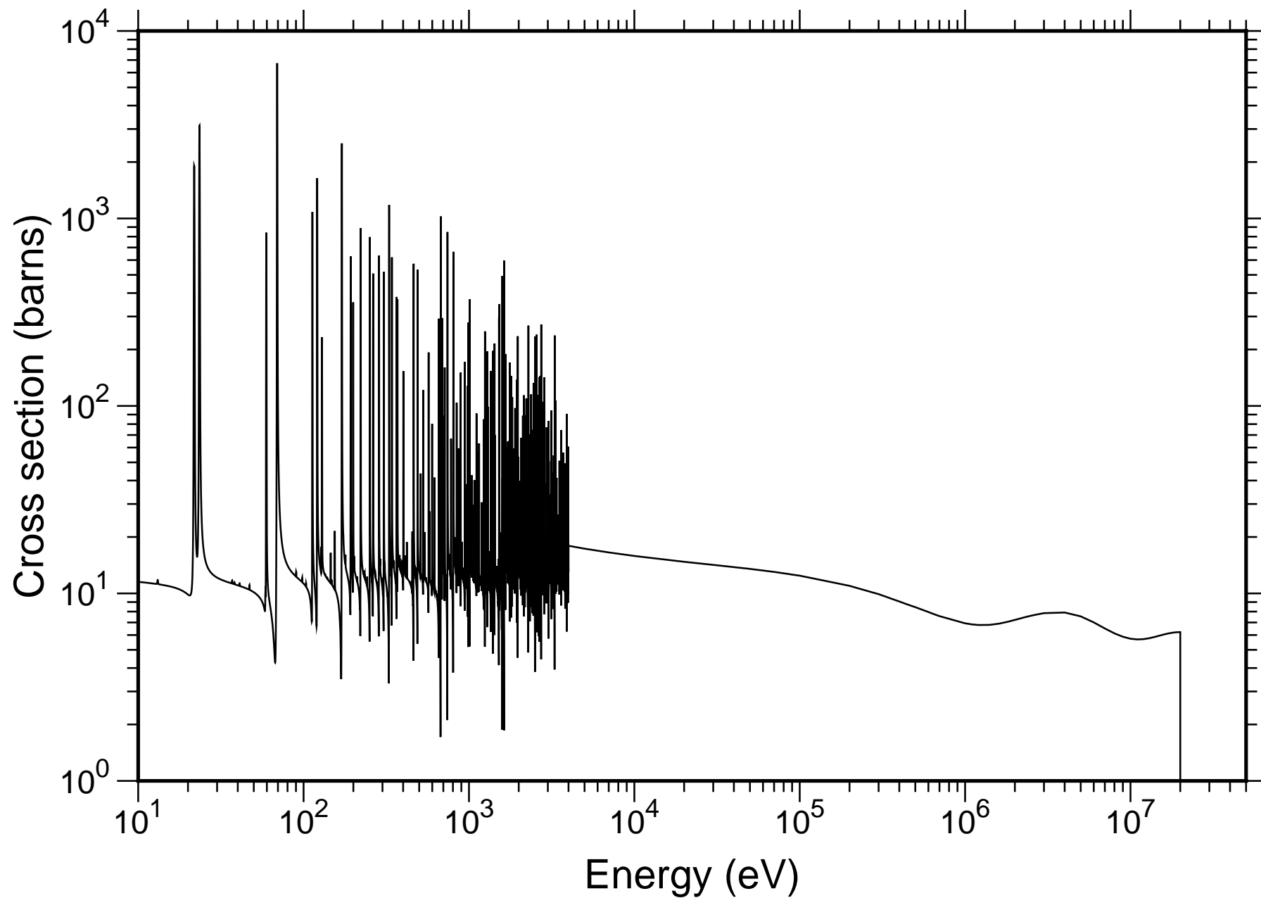
Natural Th Total Cross-section - JENDL-4.0
