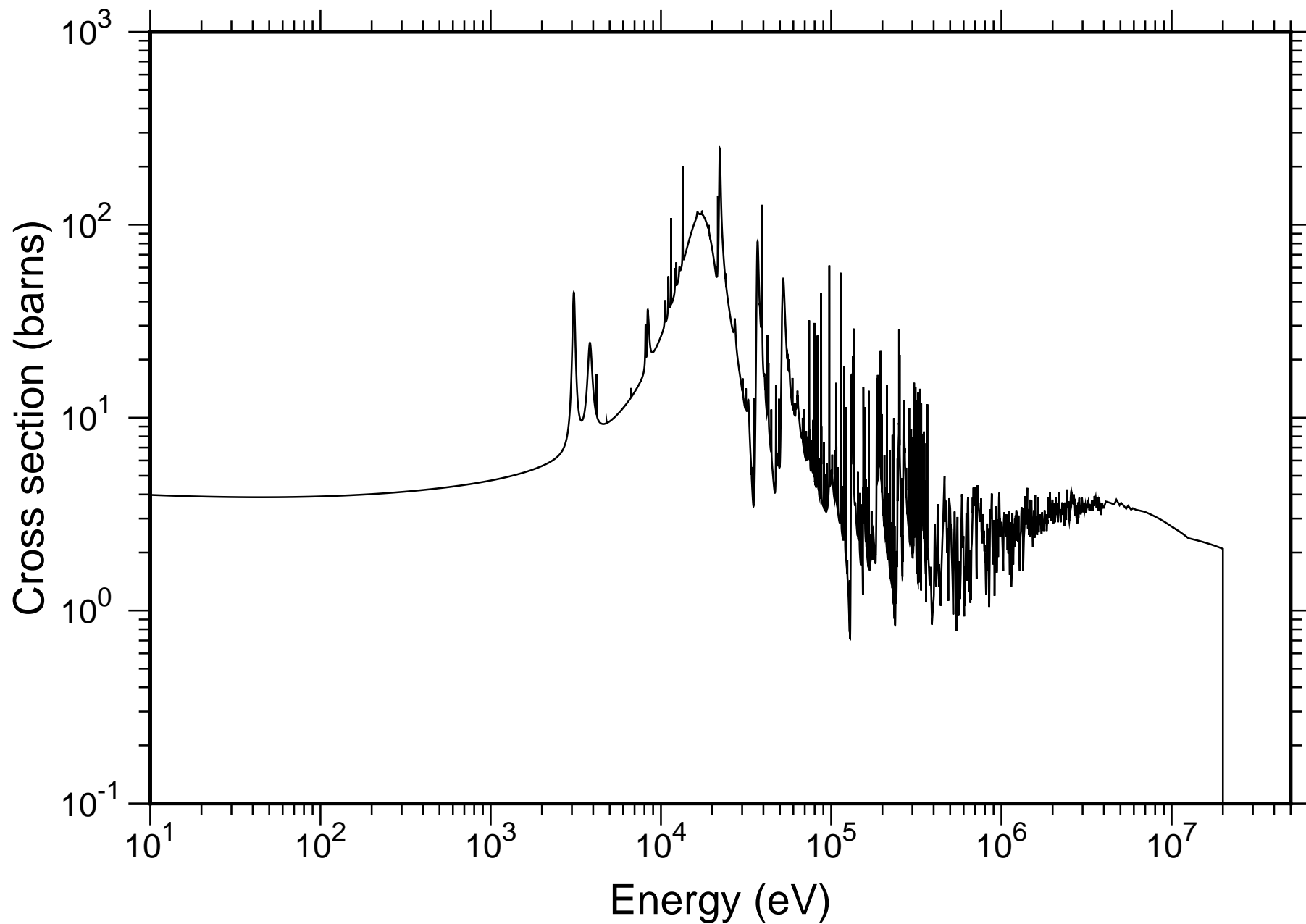
Natural Ti Total Cross-section - JENDL-4.0
