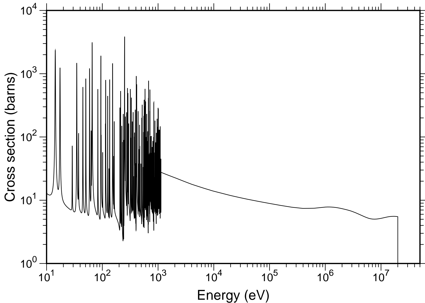
Natural Tm Total Cross-section - JENDL-4.0
