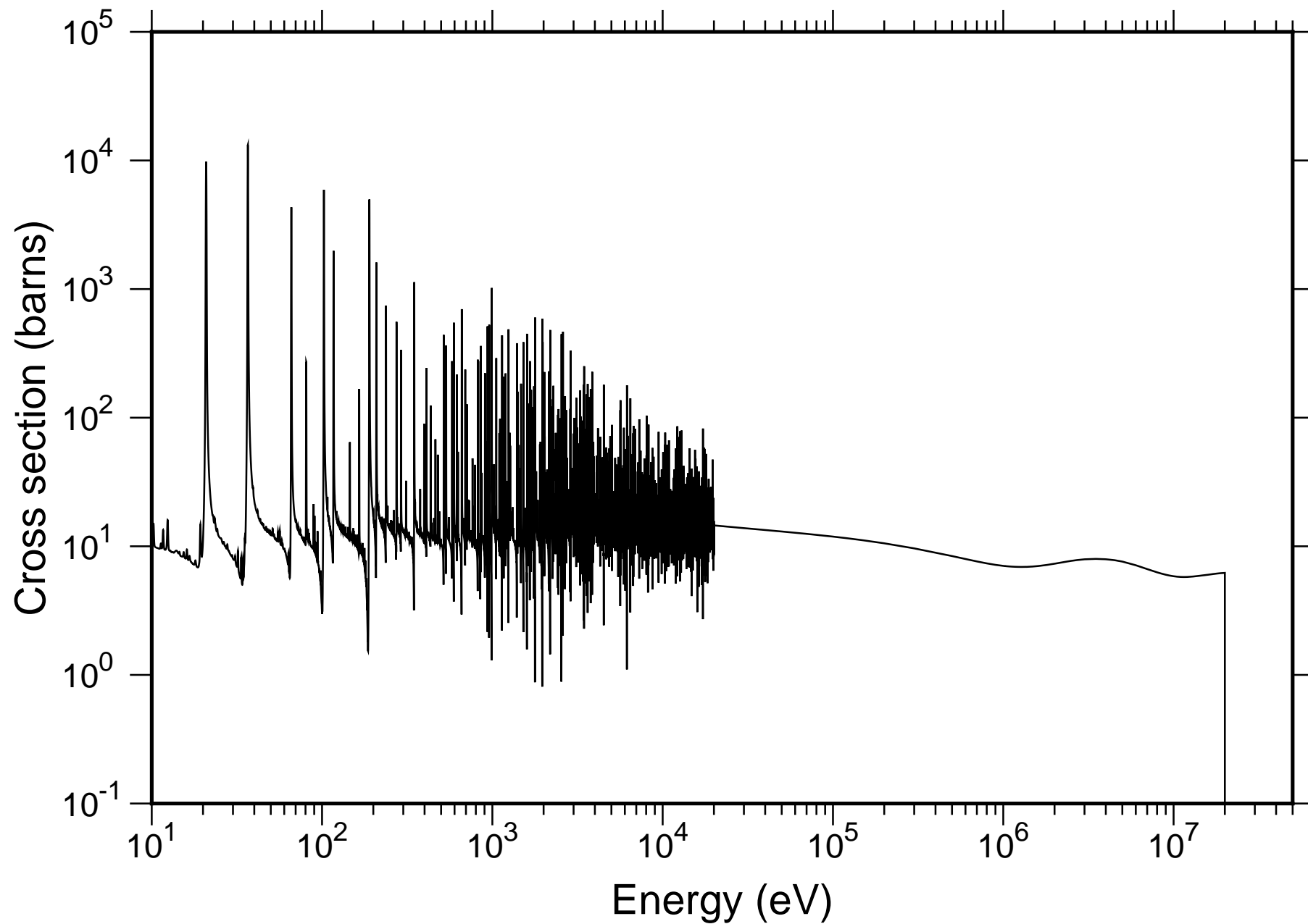
Natural U Total Cross-section - JENDL-4.0
