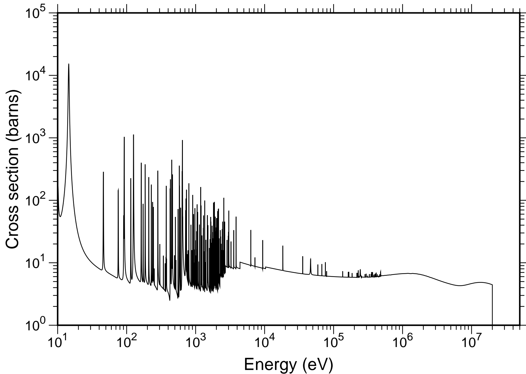
Natural Xe Total Cross-section - JENDL-4.0
