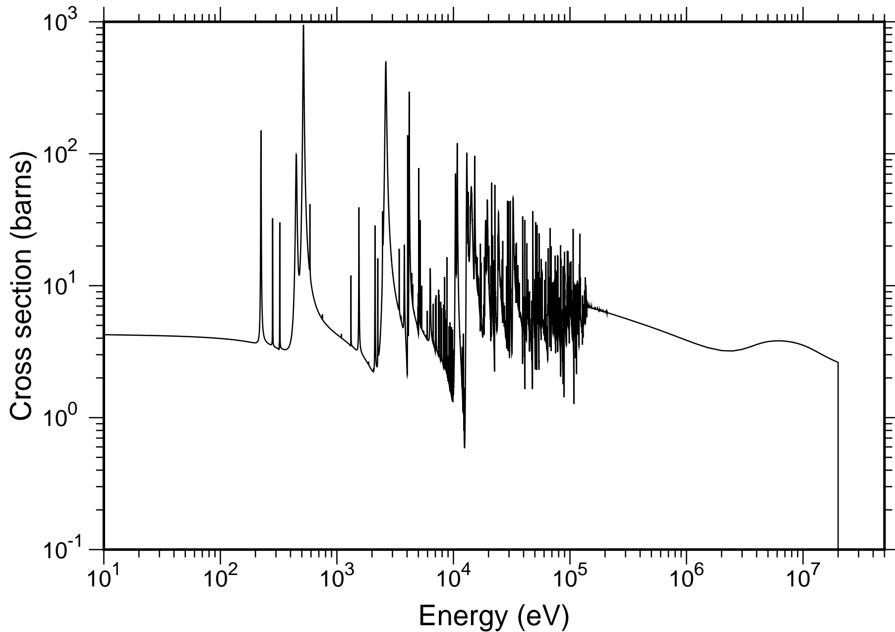
Natural Zn Total Cross-section - JENDL-4.0
