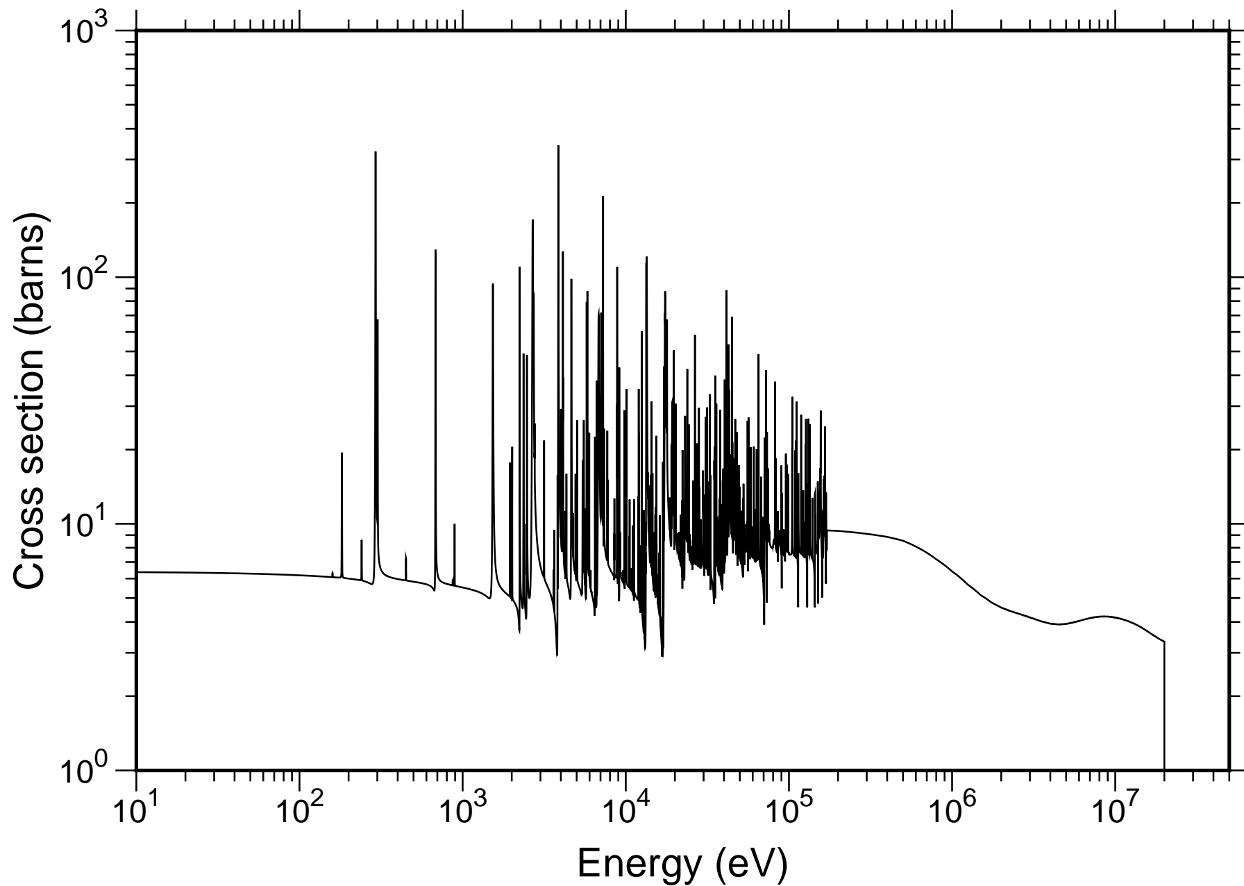
Natural Zr Total Cross-section - JENDL-4.0
