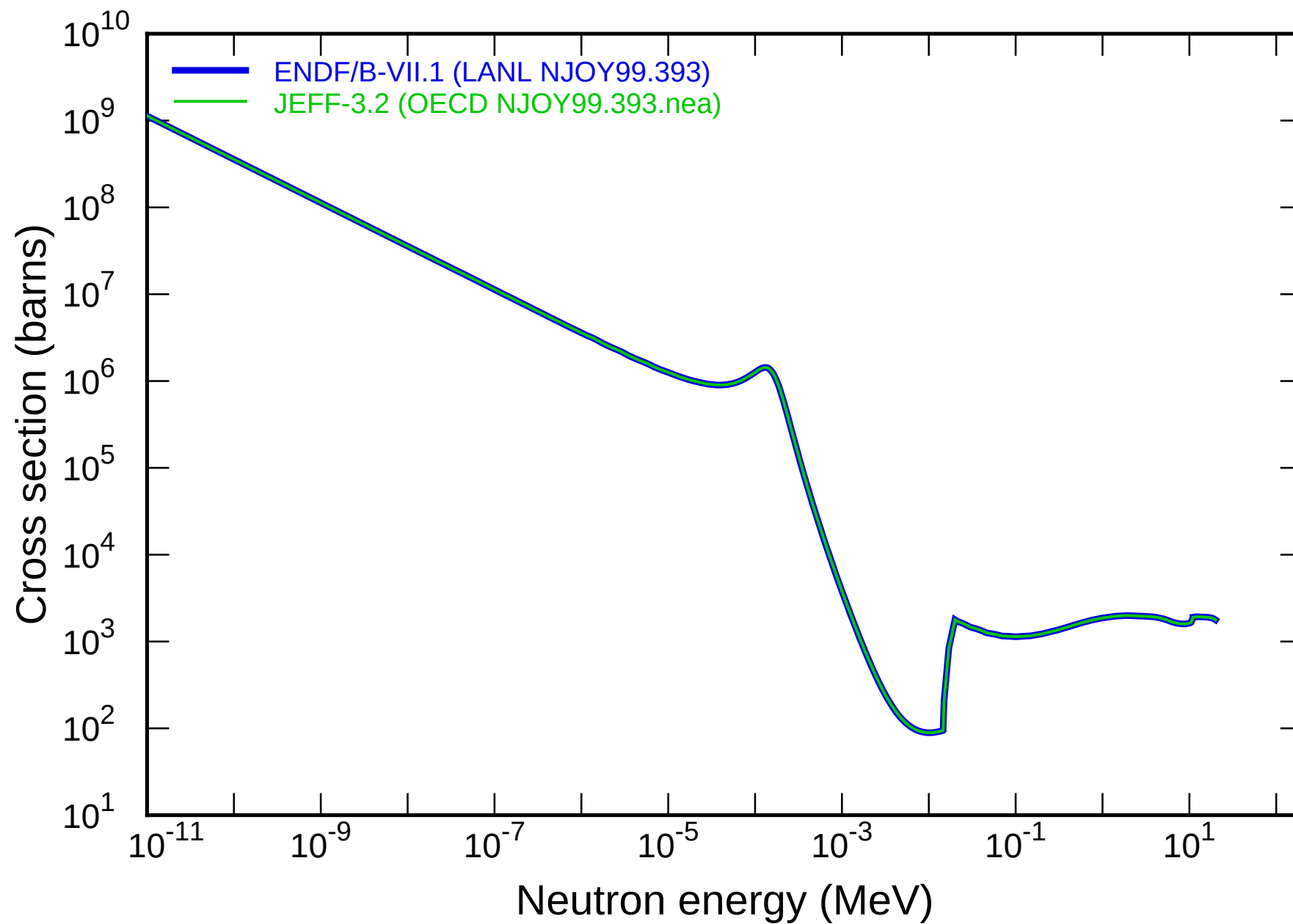
DPA cross section in ACE file of Na022
