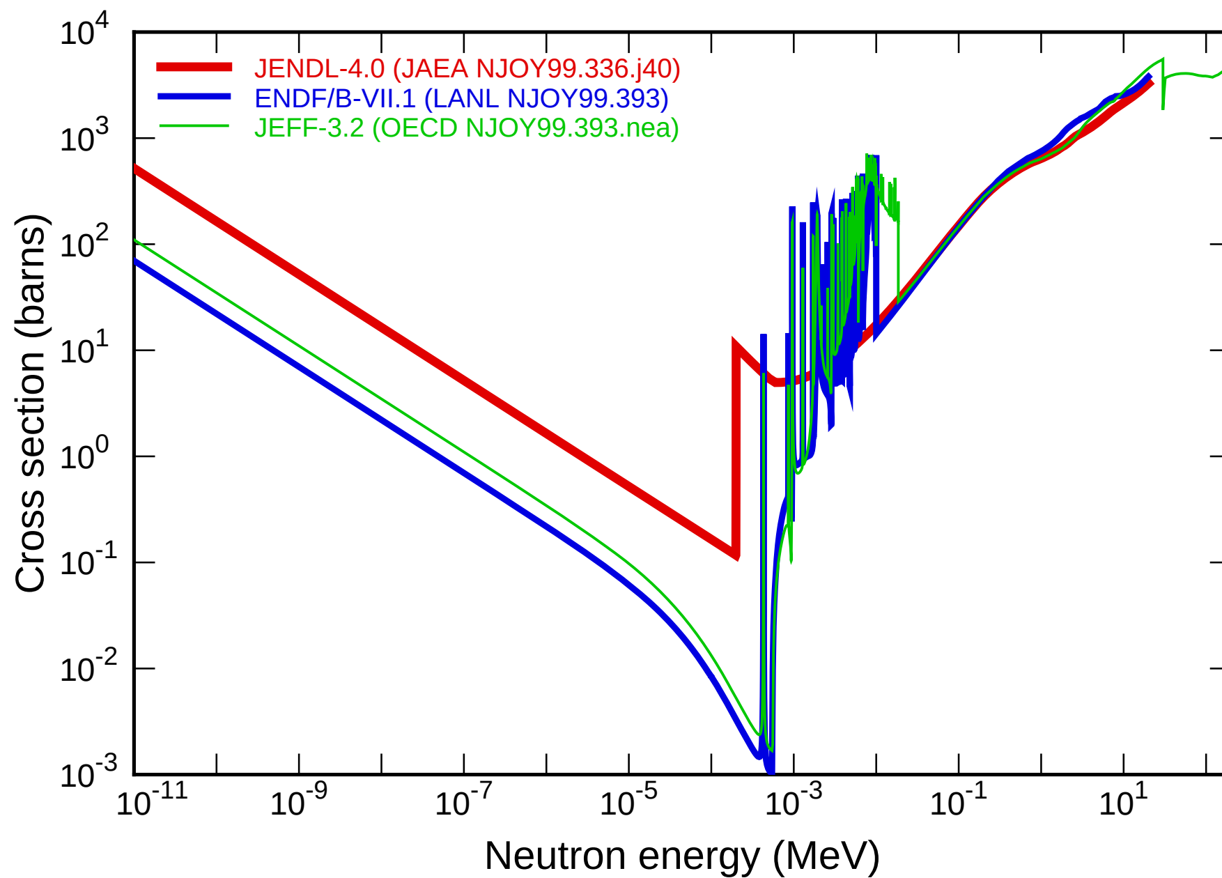
DPA cross section in ACE file of Y_090
