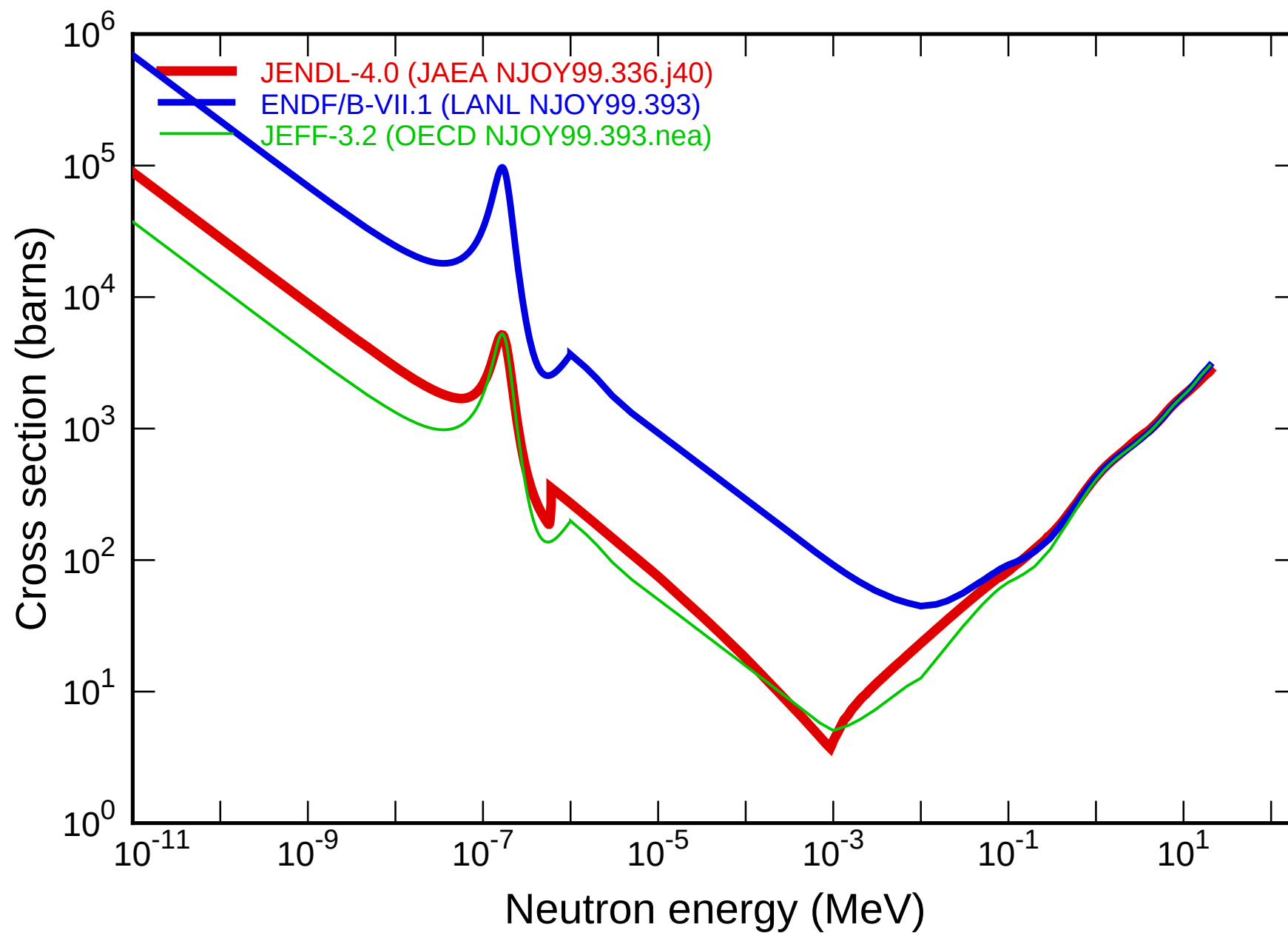
DPA cross section in ACE file of Pm148m
