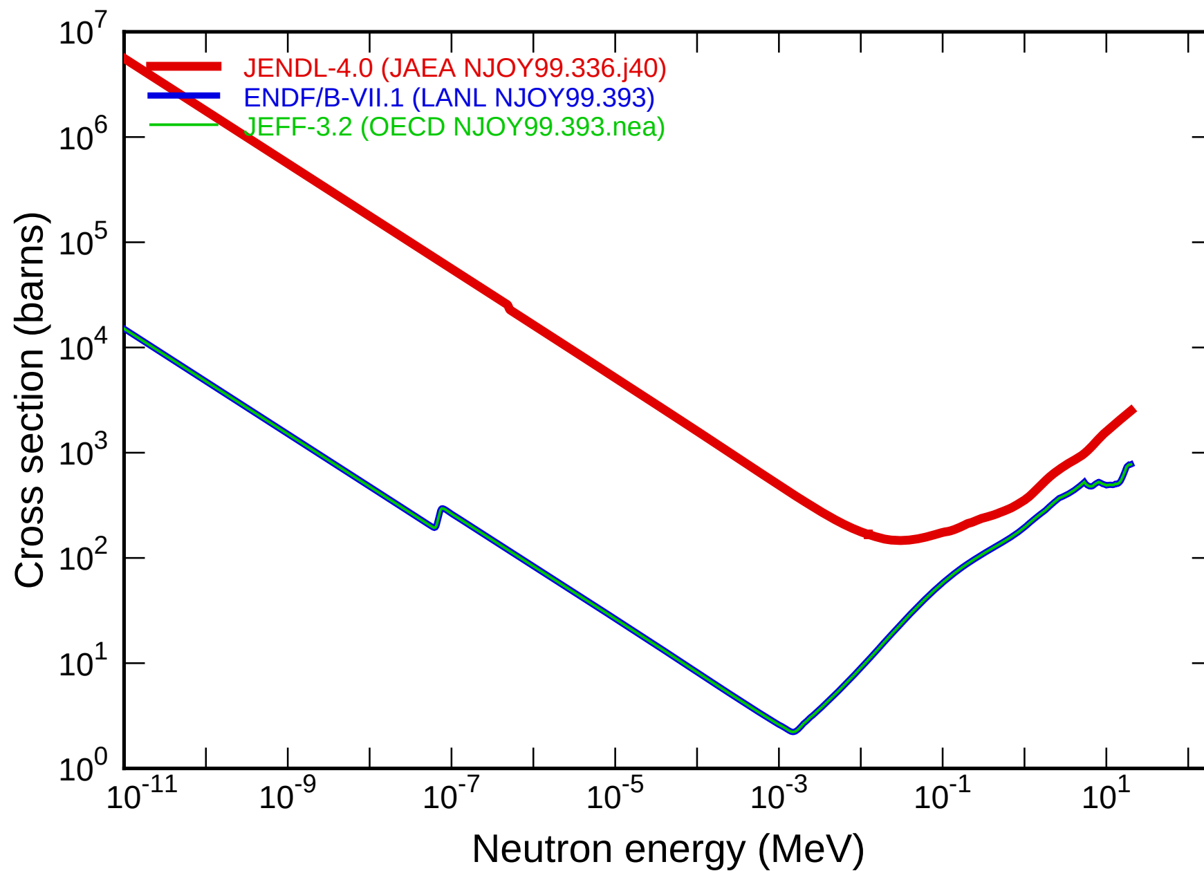
DPA cross section in ACE file of Am244m
