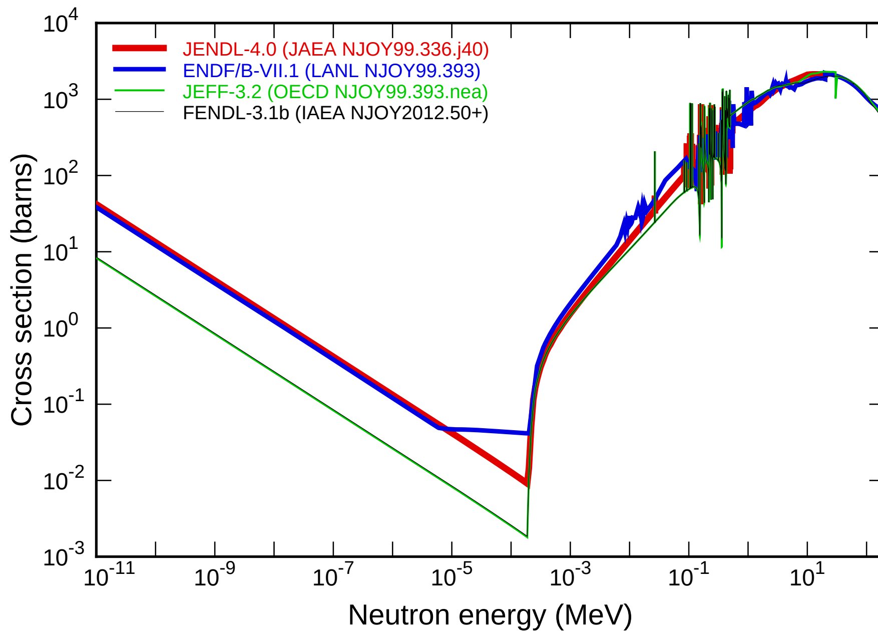
DPA cross section in ACE file of P_031
