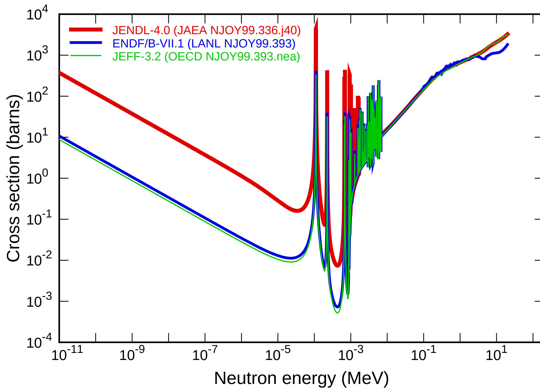
DPA cross section in ACE file of Zr093
