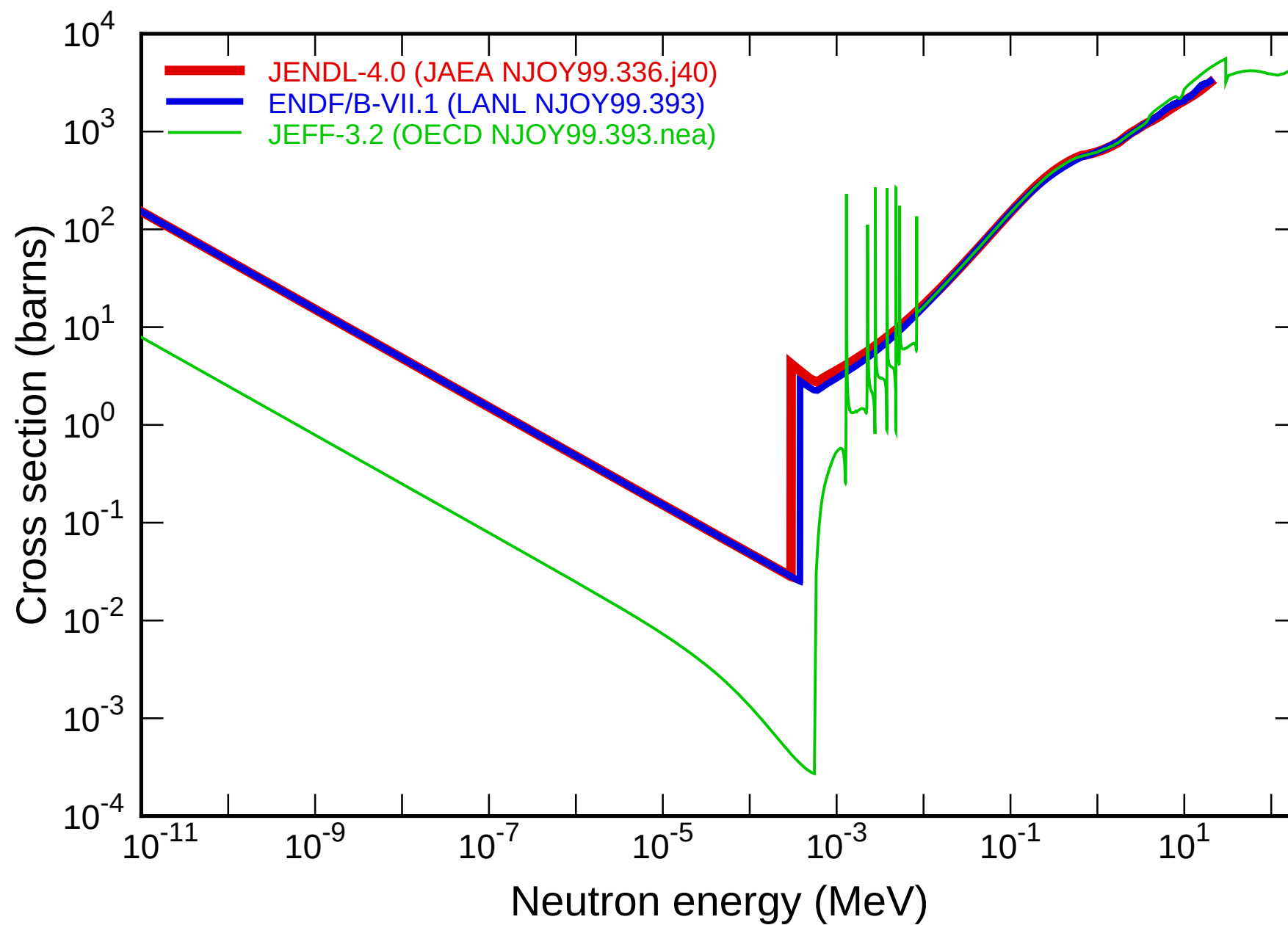
DPA cross section in ACE file of Y_091
