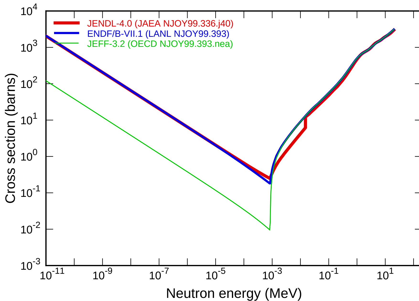
DPA cross section in ACE file of I_135
