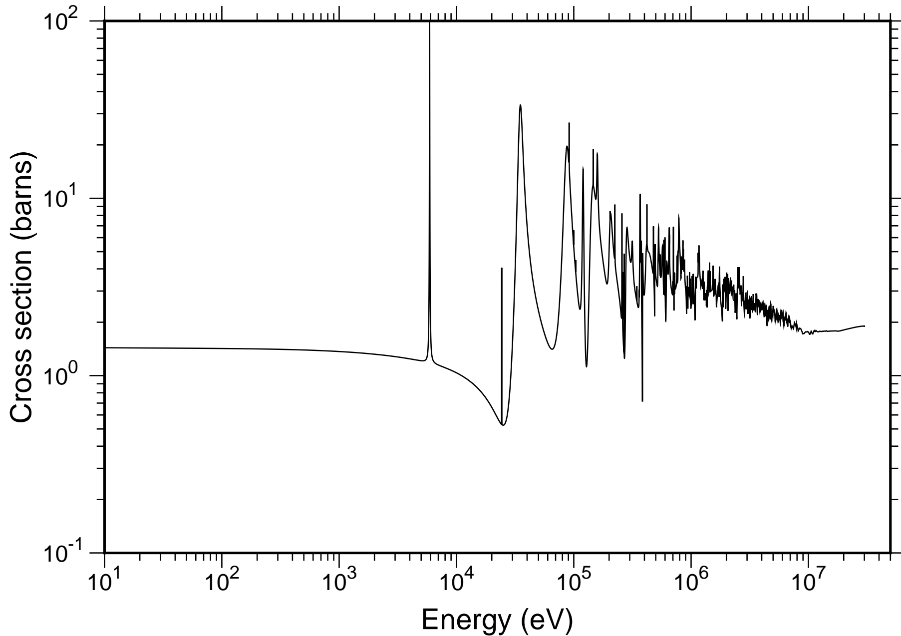
Natural Al Total Cross-section - TENDL-2019
