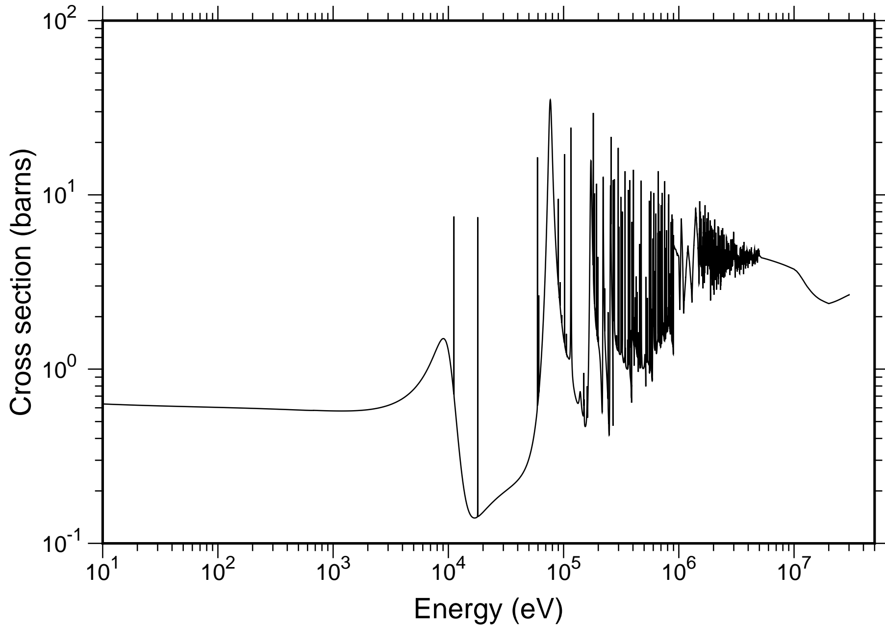
Natural Ar Total Cross-section - TENDL-2019
