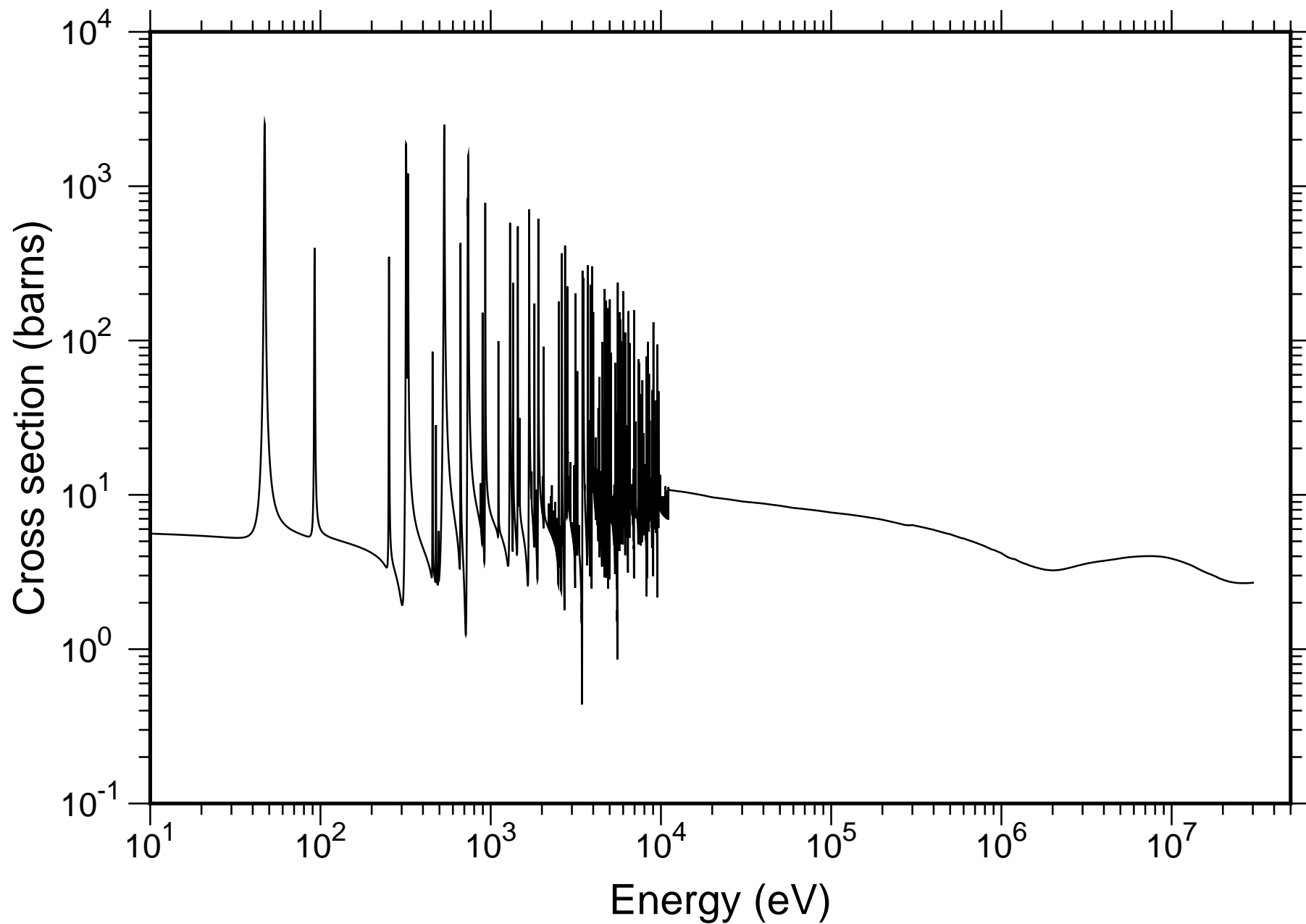
Natural As Total Cross-section - TENDL-2019
