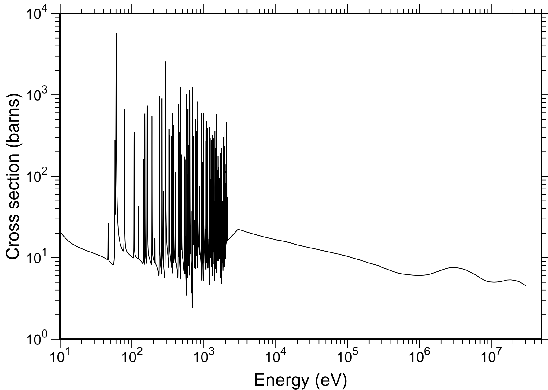
Natural Au Total Cross-section - TENDL-2019
