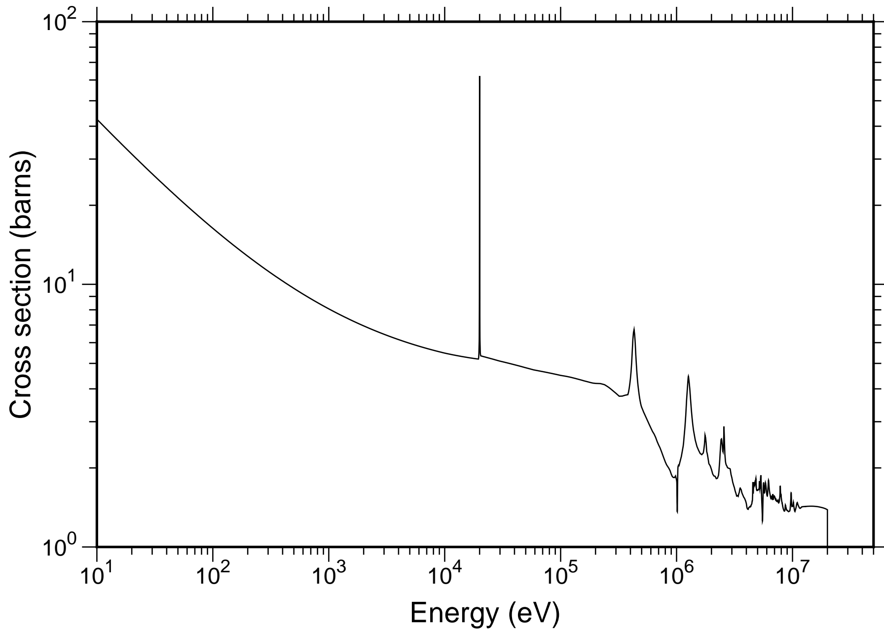
Natural B Total Cross-section - TENDL-2019
