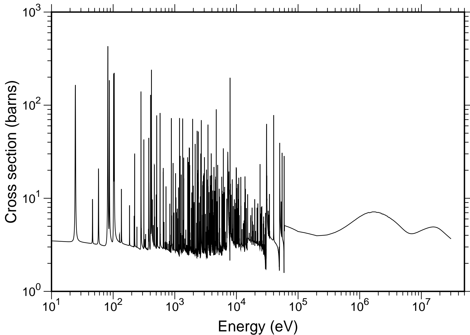
Natural Ba Total Cross-section - TENDL-2019
