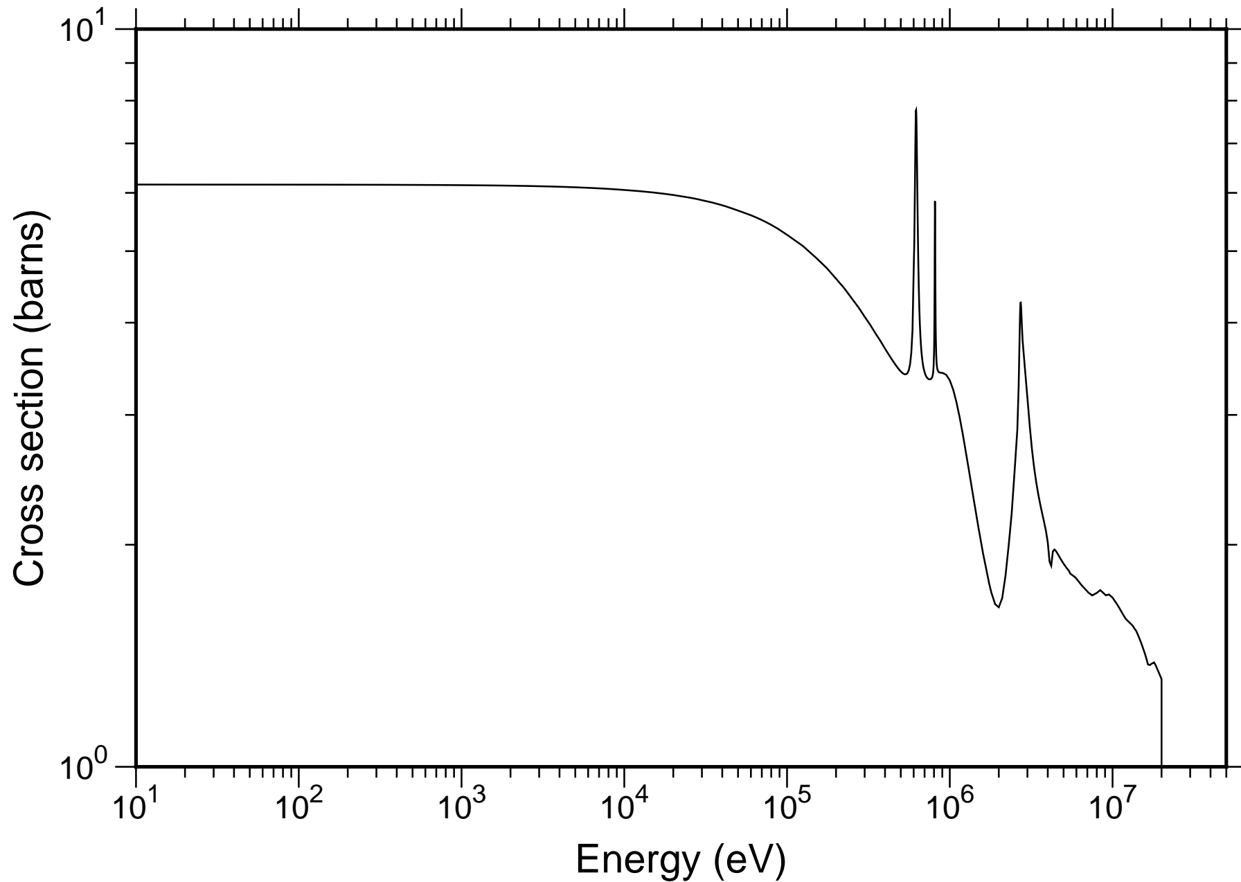
Natural Be Total Cross-section - TENDL-2019
