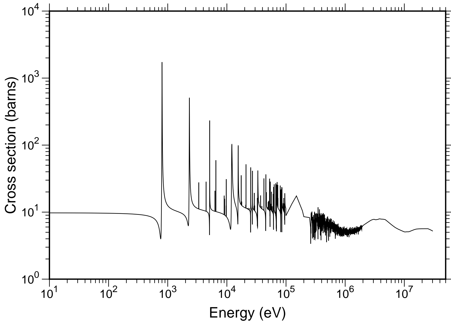
Natural Bi Total Cross-section - TENDL-2019
