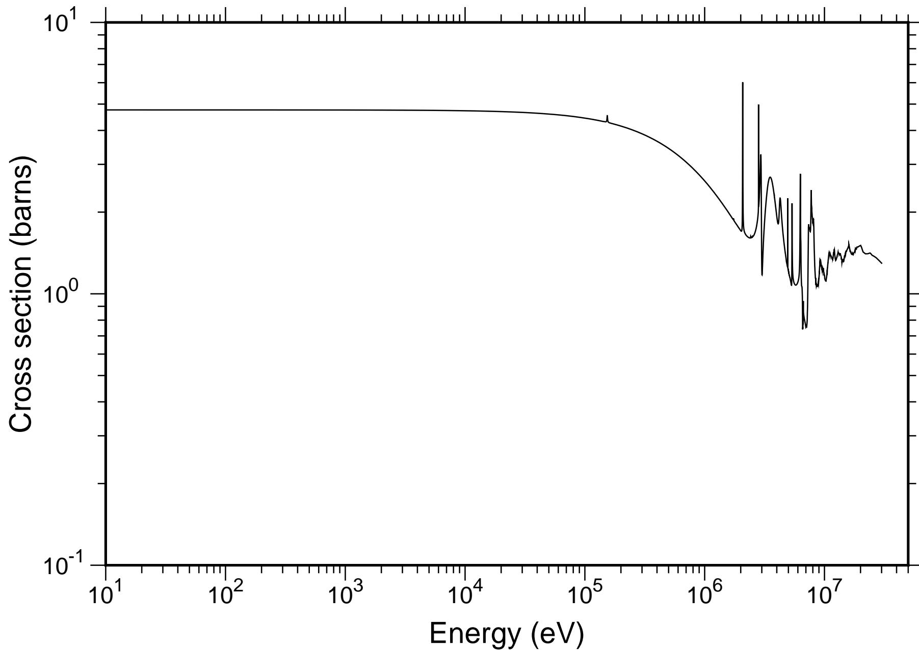
Natural C Total Cross-section - TENDL-2019
