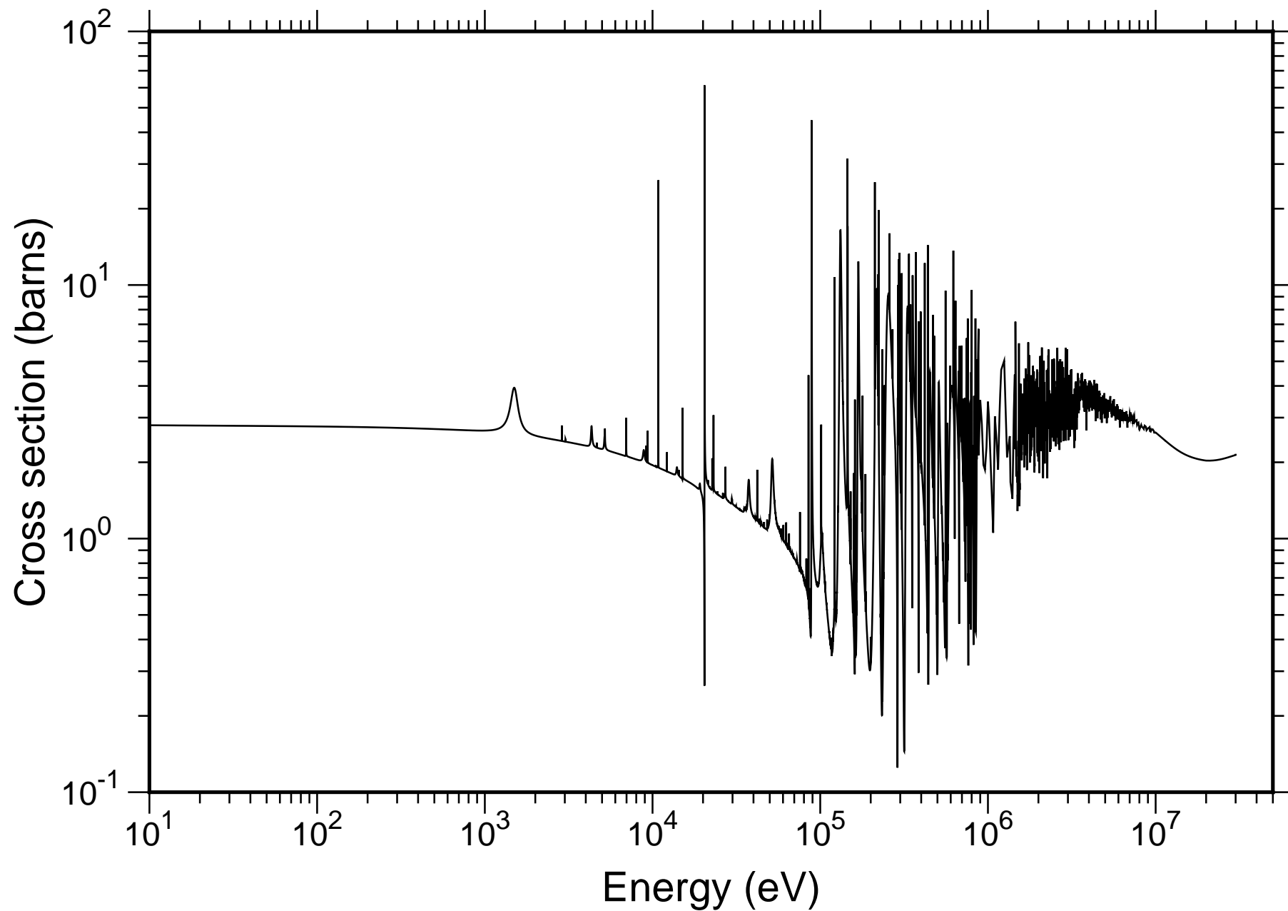
Natural Ca Total Cross-section - TENDL-2019
