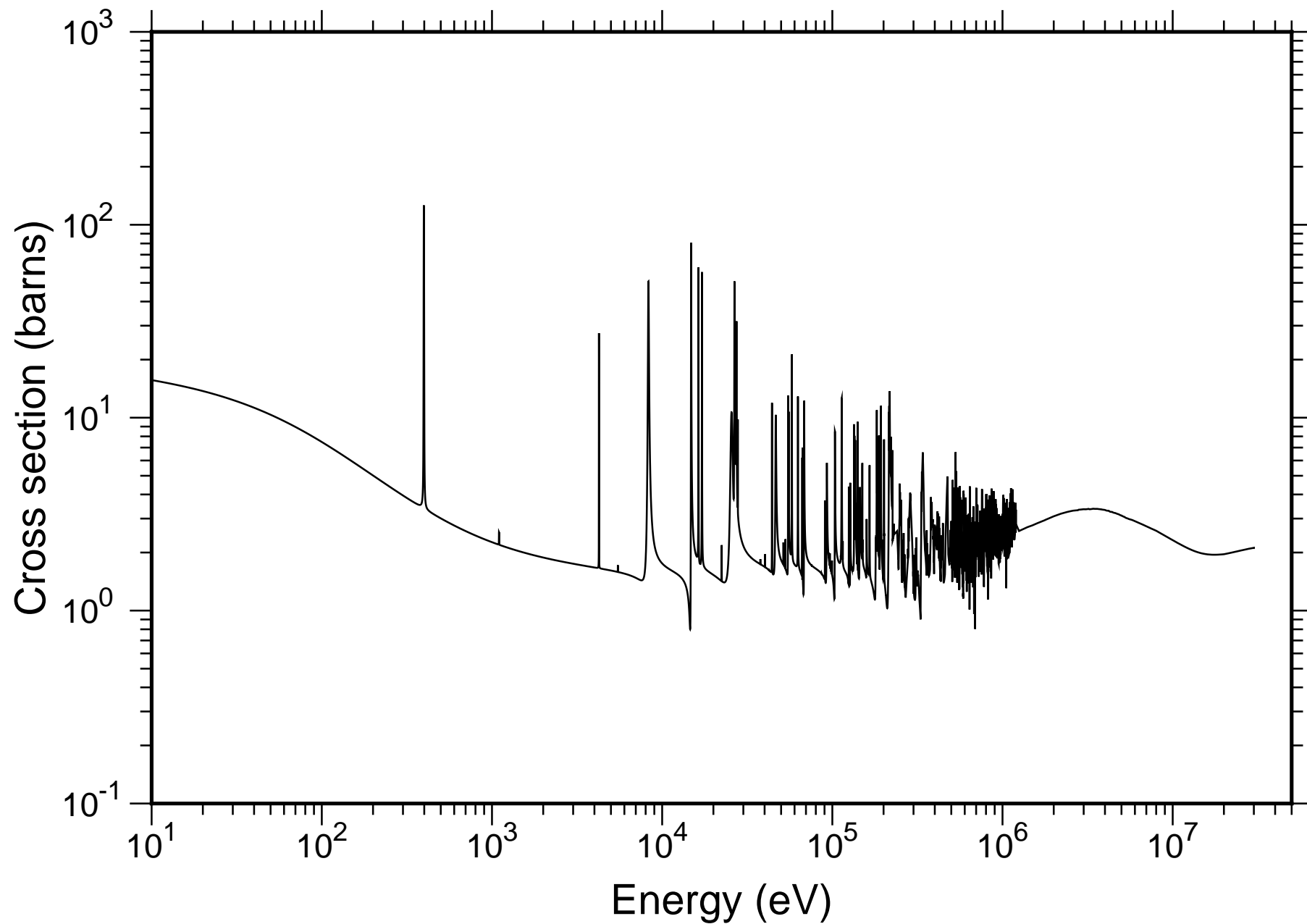
Natural Cl Total Cross-section - TENDL-2019
