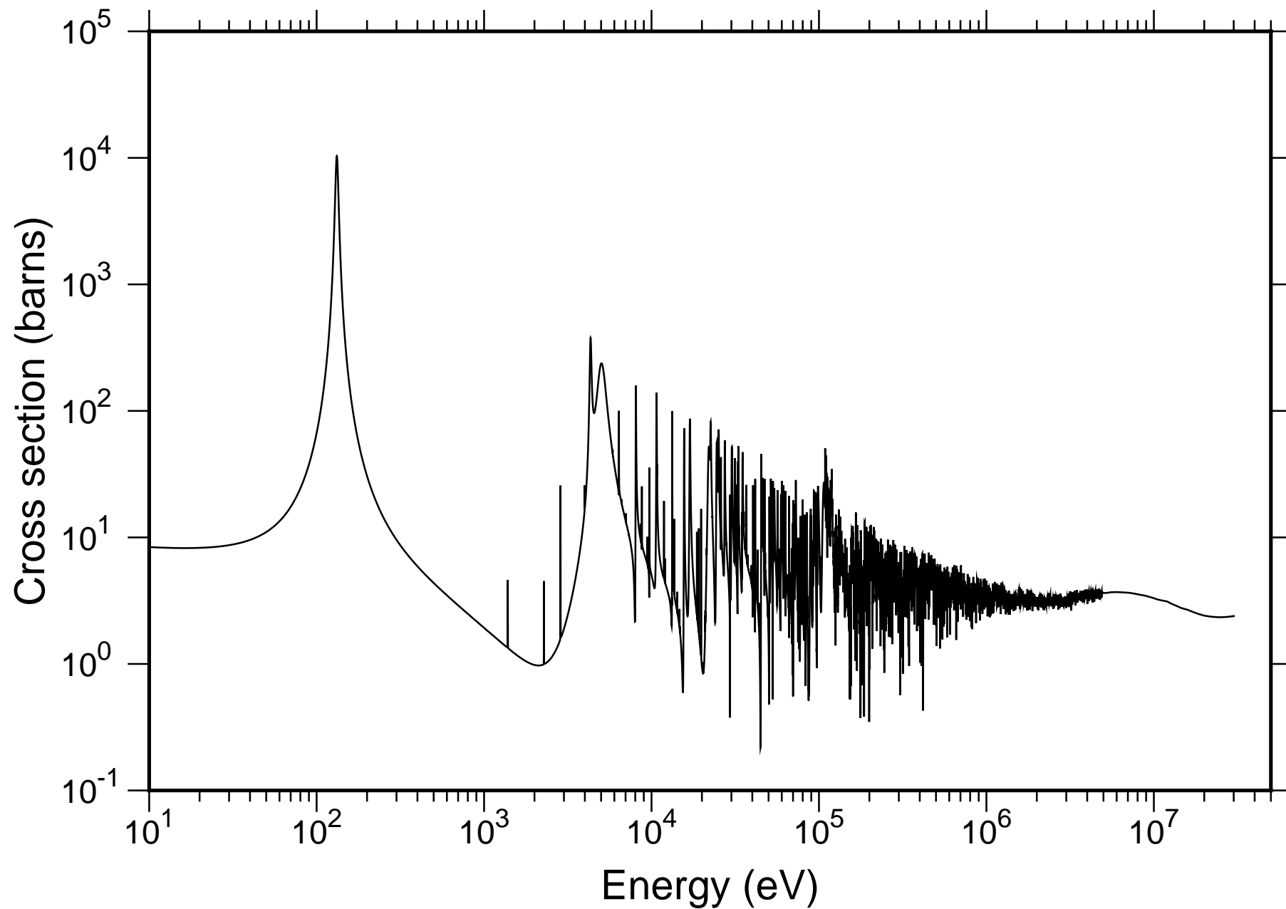
Natural Co Total Cross-section - TENDL-2019
