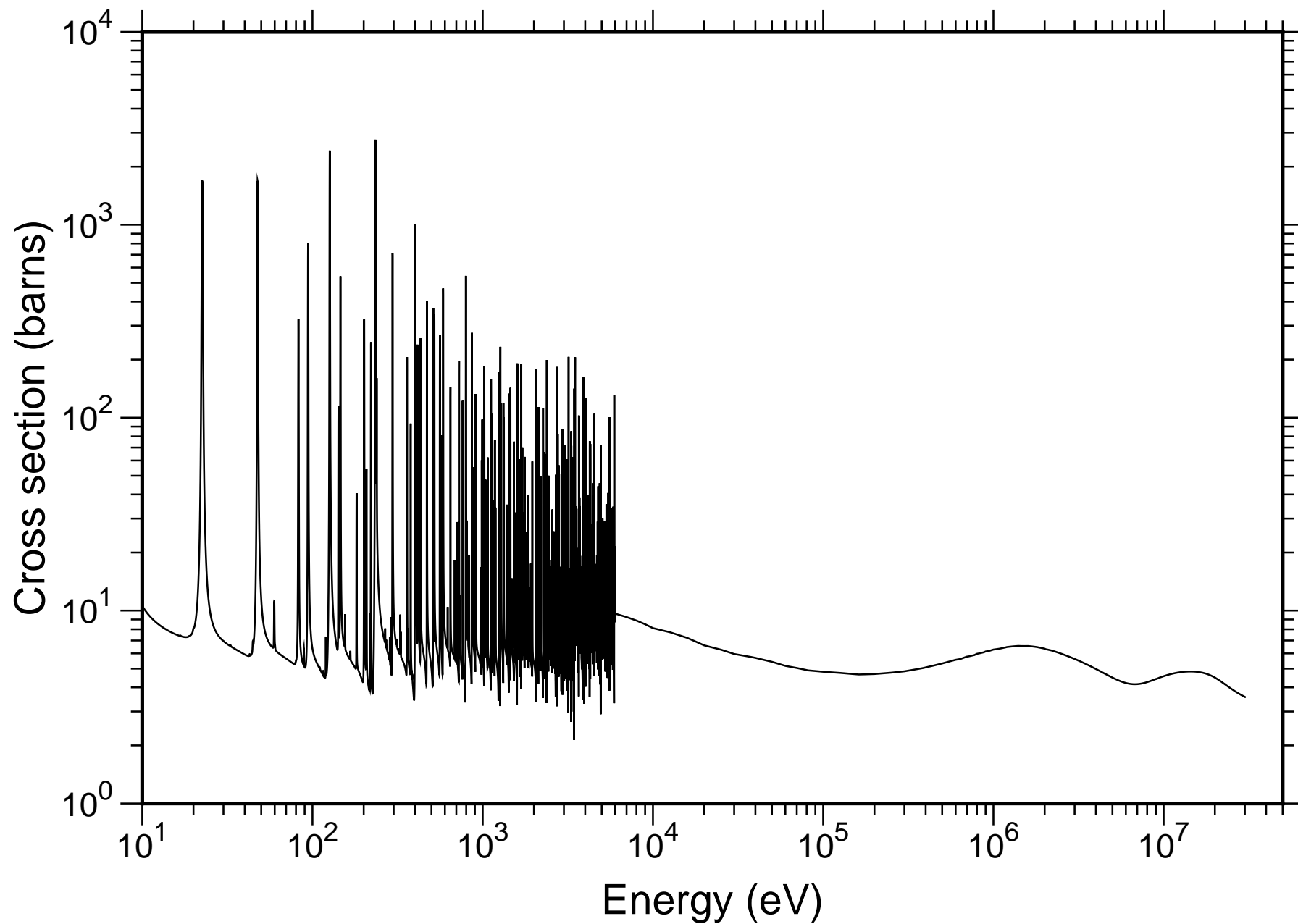
Natural Cs Total Cross-section - TENDL-2019
